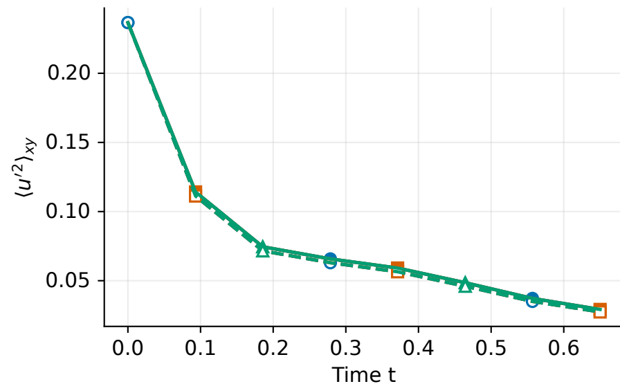
Streamwise normal stress
