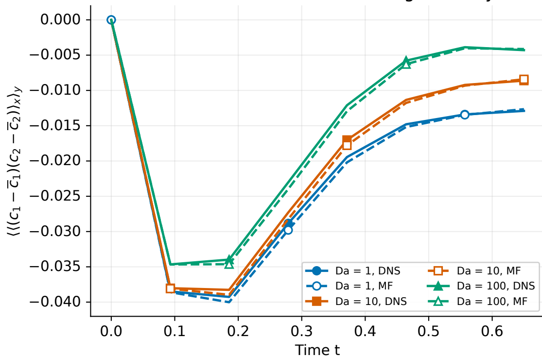
Streamwise fluctuations, averaged over y
