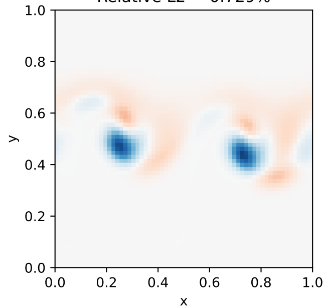
MF — DNS Relative L2 = 0.729%
