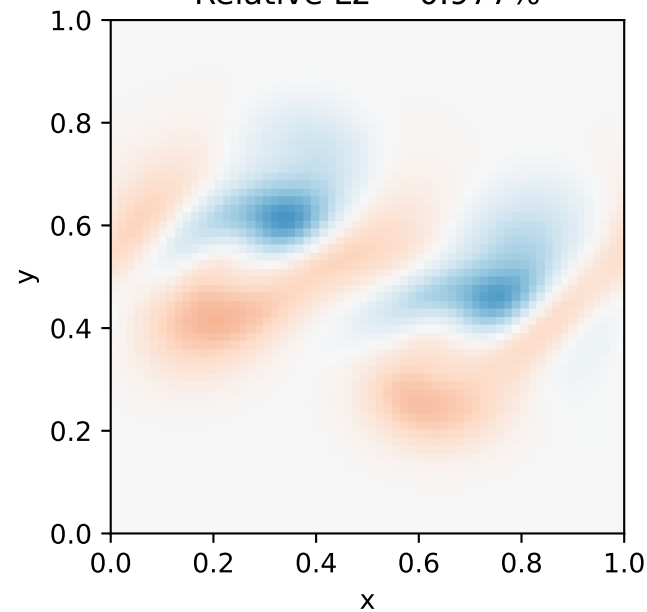
MF — DNS Relative L2 = 0.977%
