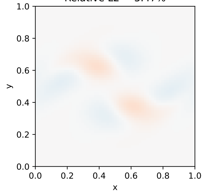
MF — DNS Relative L2 = 3.47%
