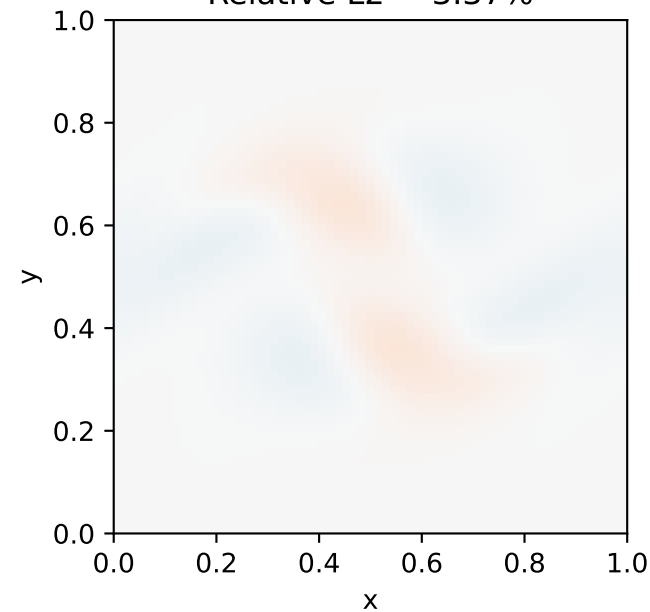
MF — DNS Relative L2 = 3.37%
