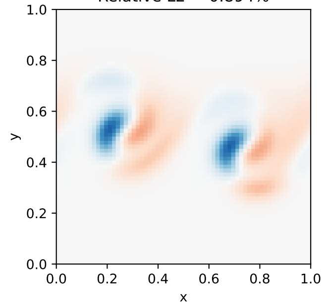
MF — DNS Relative L2 = 0.894%
