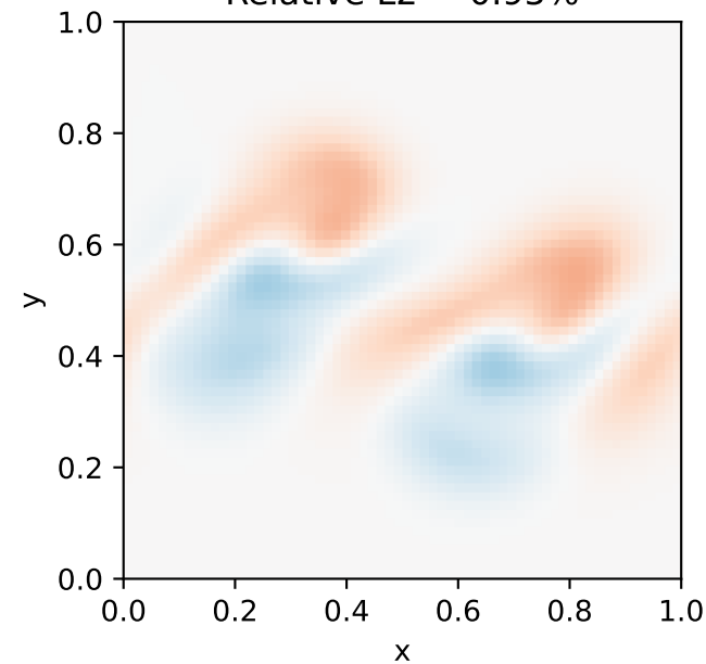
MF — DNS Relative L2 = 0.95%
