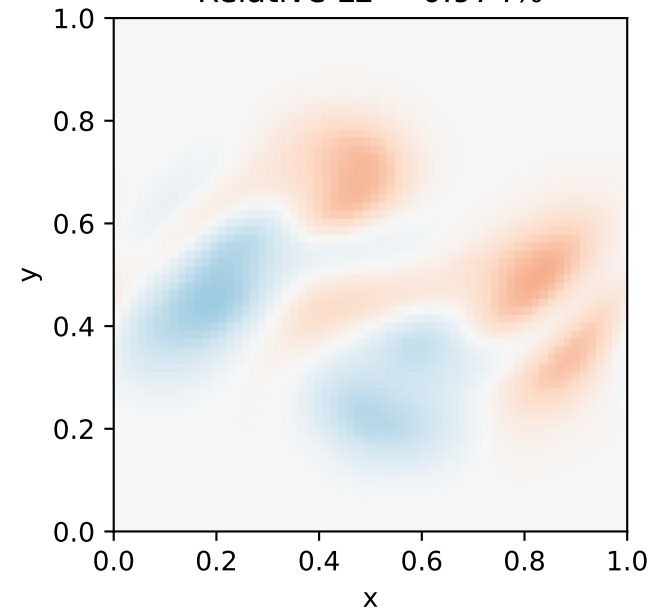
MF — DNS Relative L2 = 0.974%
