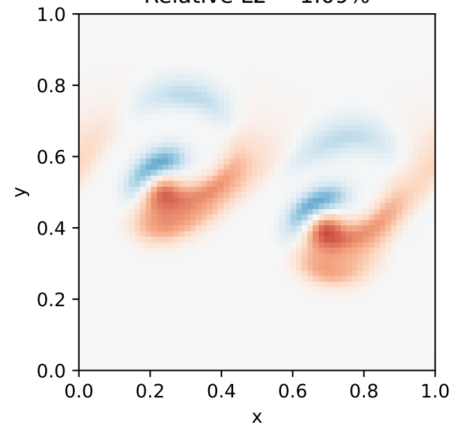
MF — DNS Relative L2 = 1.09%
