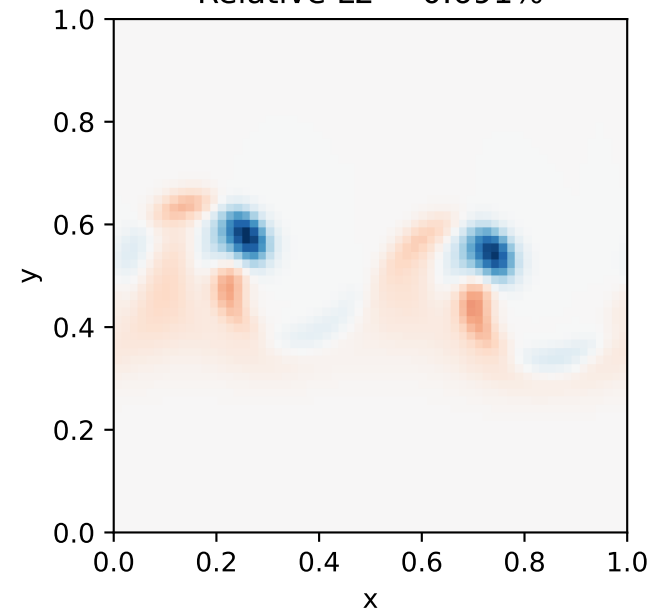
MF - DNS Relative L2 = 0.691%
