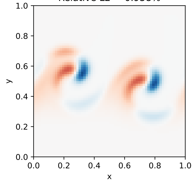
MF - DNS Relative L2 = 0.958%
