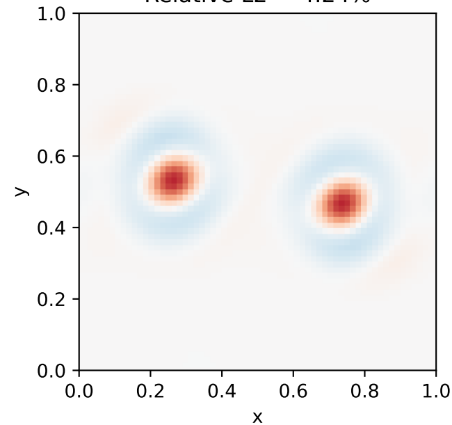
MF — DNS Relative L2 = 4.24%
