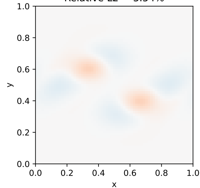
MF — DNS Relative L2 = 3.54%
