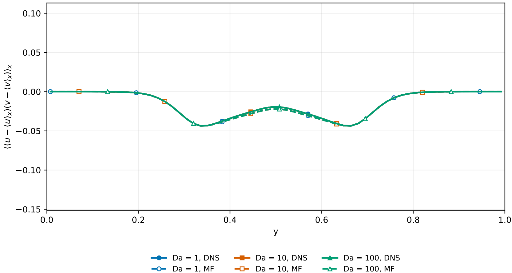
Reynolds shear stress vs y 64×64, Re = Pe = 100, RK4; t = 0.093125
