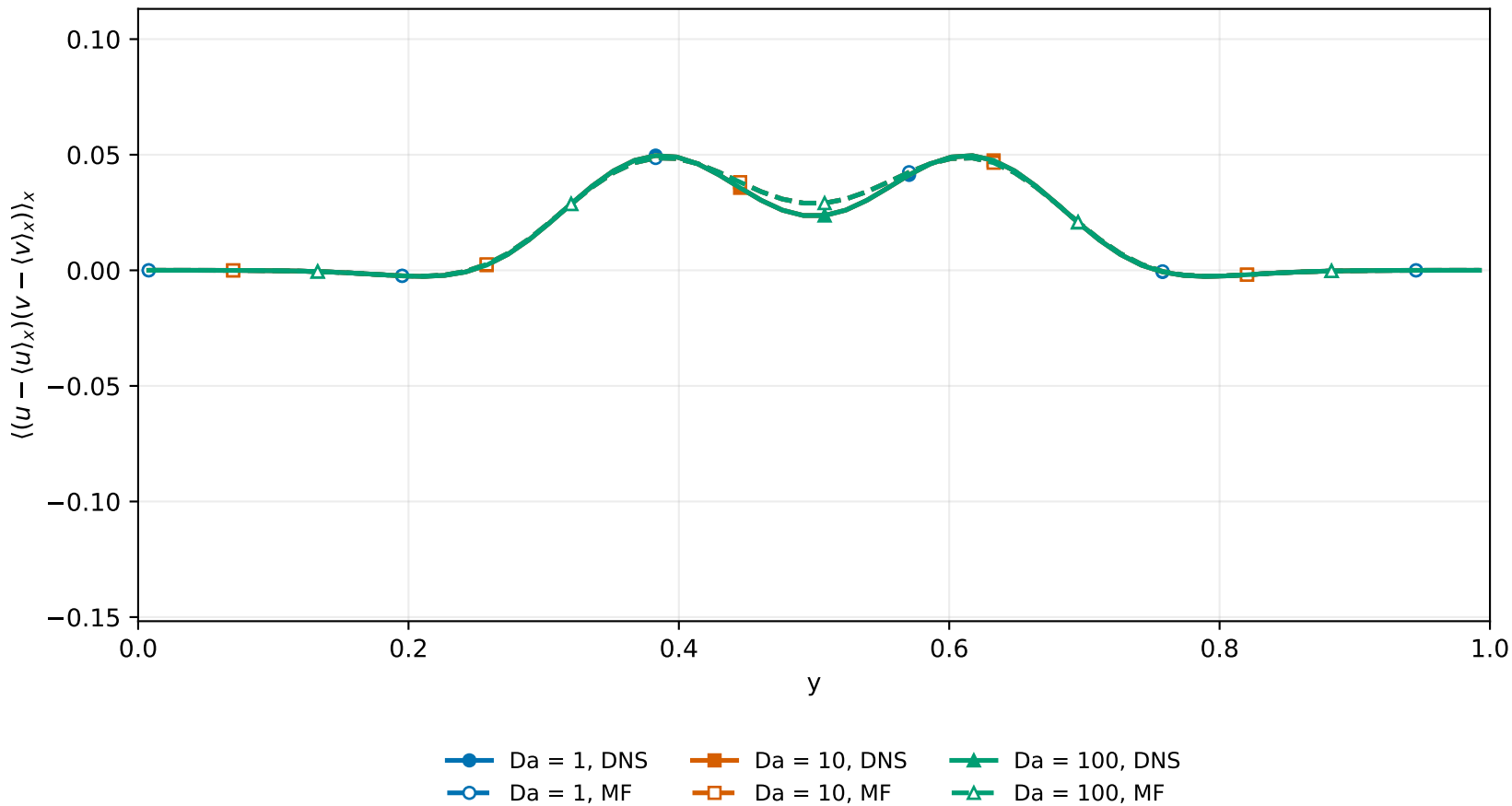
Reynolds shear stress vs y 64×64, Re = Pe = 100, RK4; t = 0.278750
