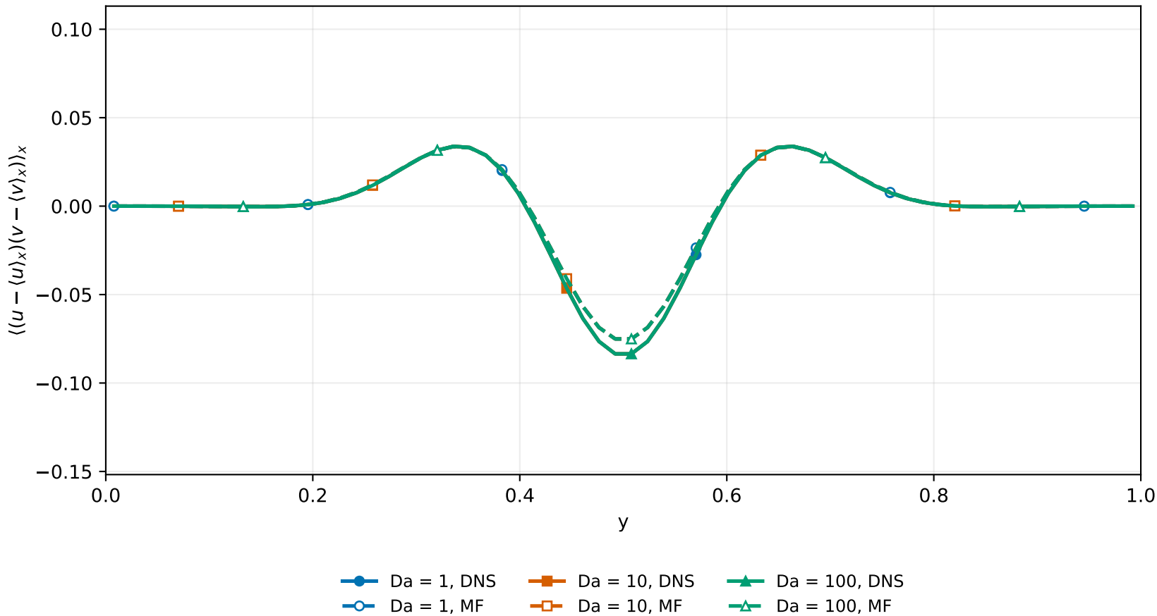
Reynolds shear stress vs y 64×64, Re = Pe = 100, RK4; t = 0.371250
