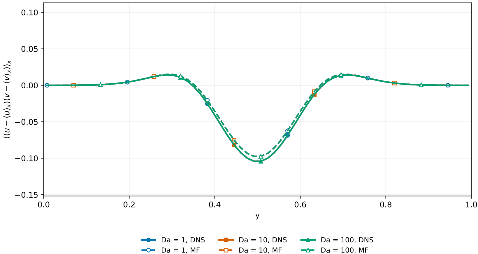
Reynolds shear stress vs y 64×64, Re = Pe = 100, RK4; t = 0.556875
