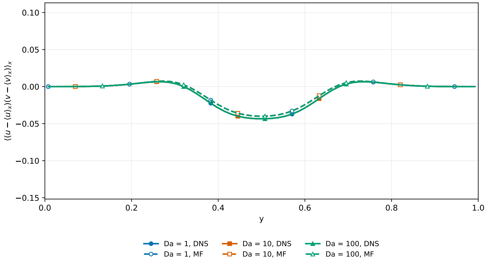
Reynolds shear stress vs y 64×64, Re = Pe = 100, RK4; t = 0.650000
