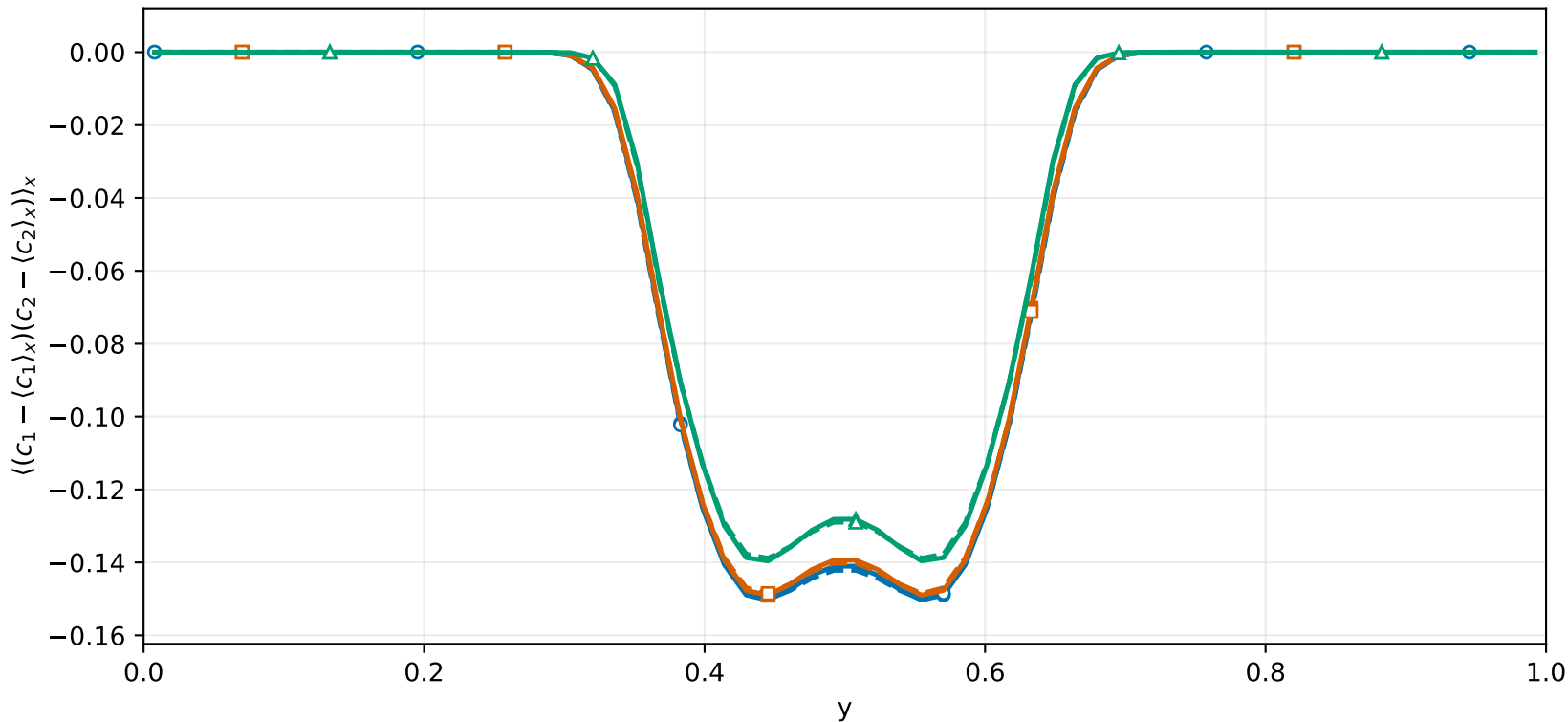
Unmixedness (signed covariance) vs y 64 \times 64 , Re = Pe = 100 , RK4; t = 0.093125
