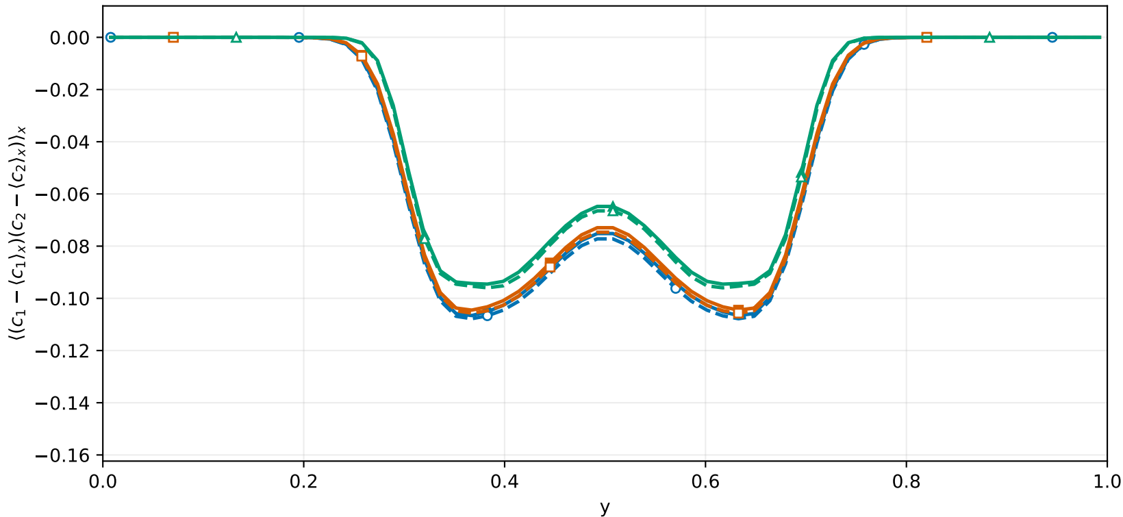
Unmixedness (signed covariance) vs y 64 \times 64 , Re = Pe = 100 , RK4; t = 0.185625
