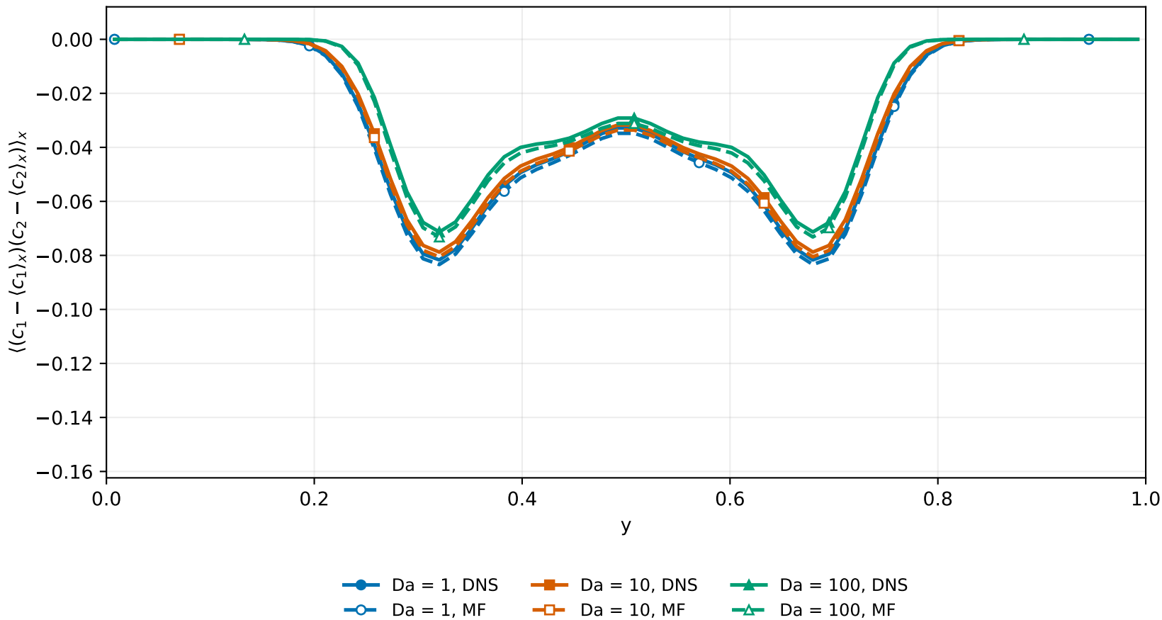
Unmixedness (signed covariance) vs y 64 \times 64 , Re = Pe = 100 , RK4; t = 0.278750
