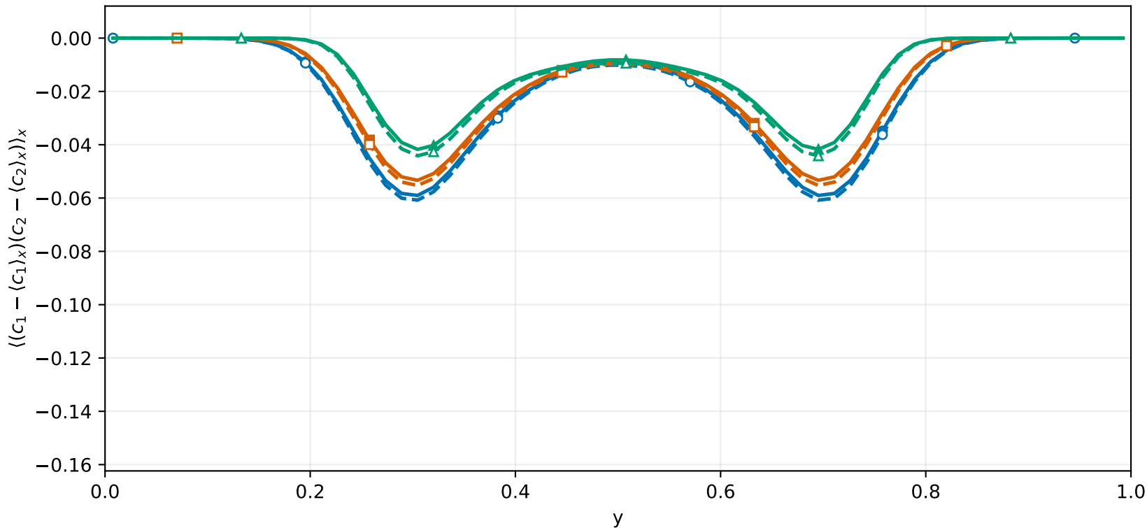
Unmixedness (signed covariance) vs y 64 \times 64 , Re = Pe = 100 , RK4; t = 0.371250
