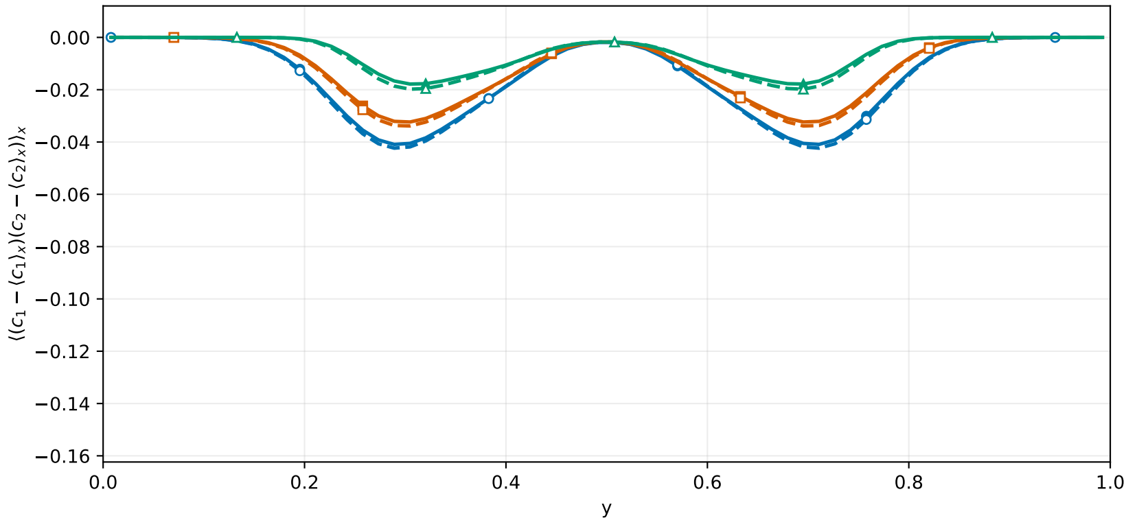
Unmixedness (signed covariance) vs y 64 \times 64 , Re = Pe = 100 , RK4; t = 0.464375
