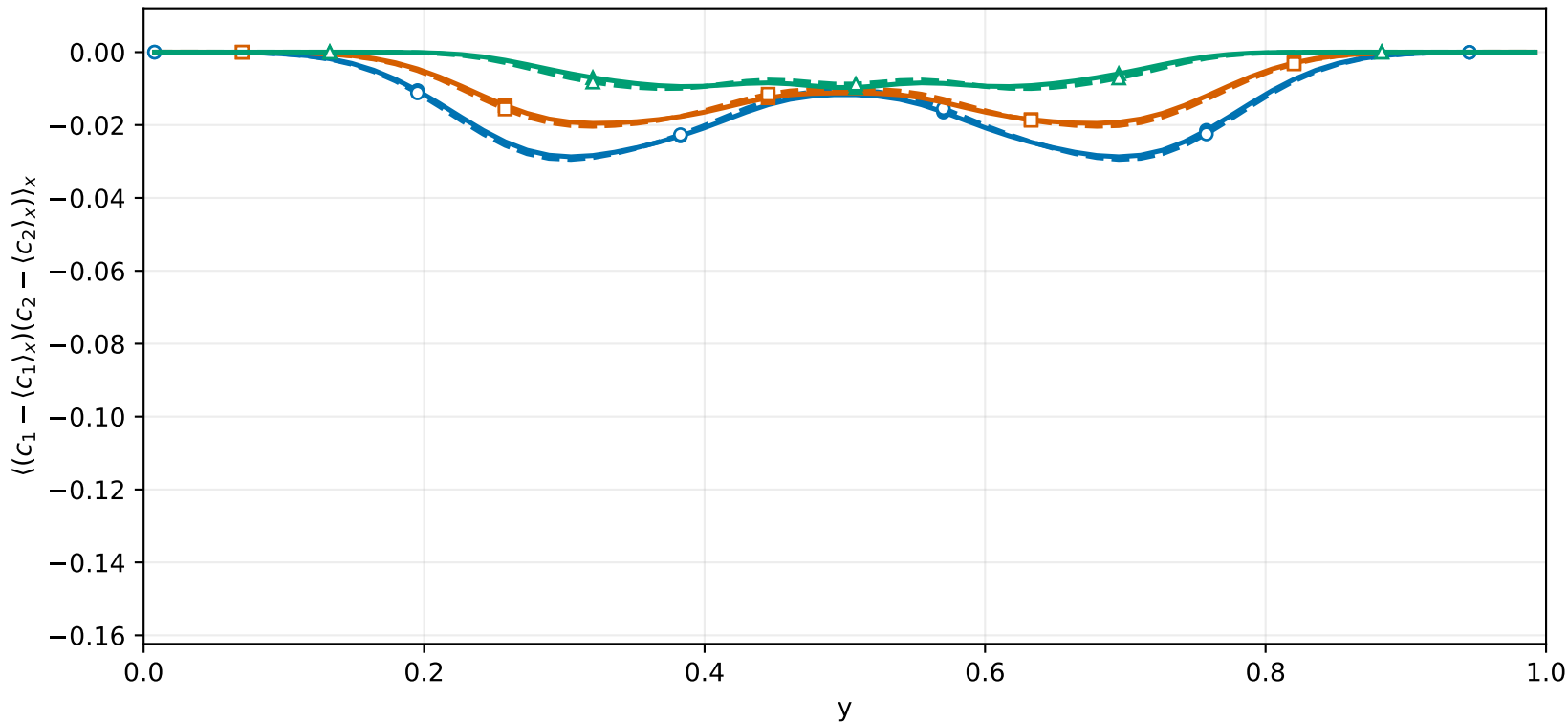
Unmixedness (signed covariance) vs y 64×64, Re = Pe = 100, RK4; t = 0.556875
