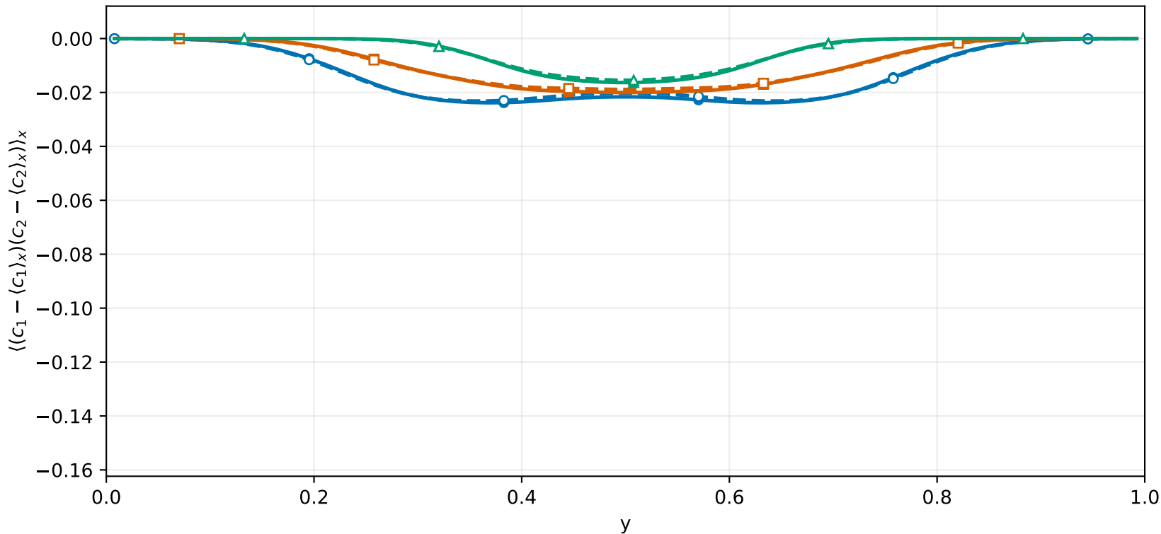
Unmixedness (signed covariance) vs y 64 \times 64 , Re = Pe = 100 , RK4; t = 0.650000
