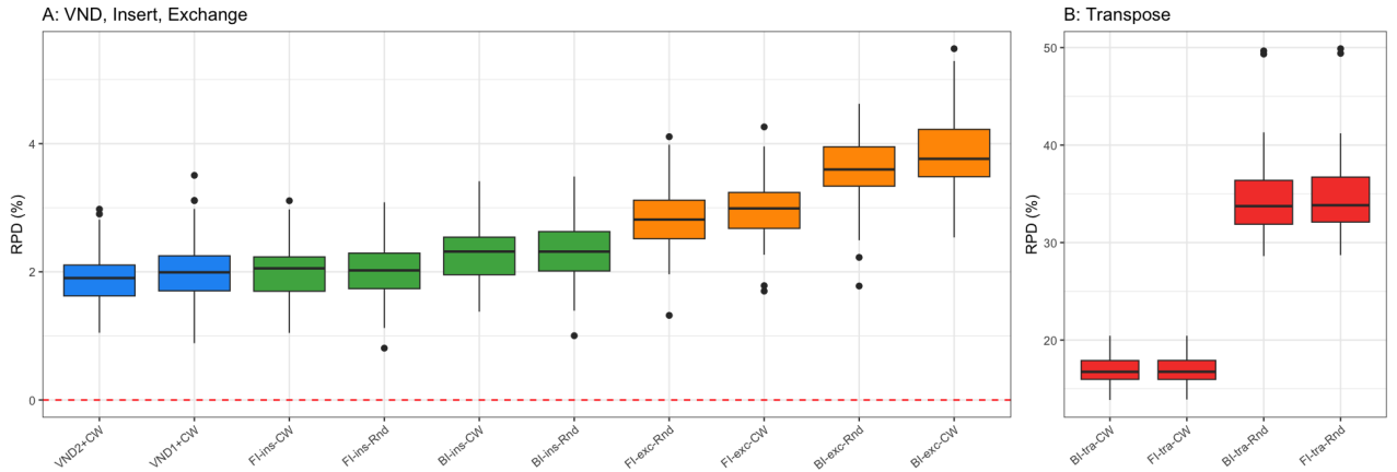
FIGURE 4.2: RPD distribution across the 78 instances. Panel A shows the competitive algorithms (scale 0–6%); Panel B shows transpose on a larger scale (15–45%) to make the spread visible.
