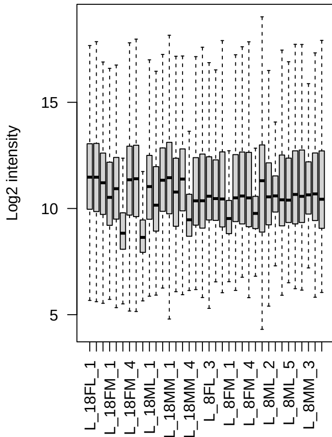
After MinProb imputation
