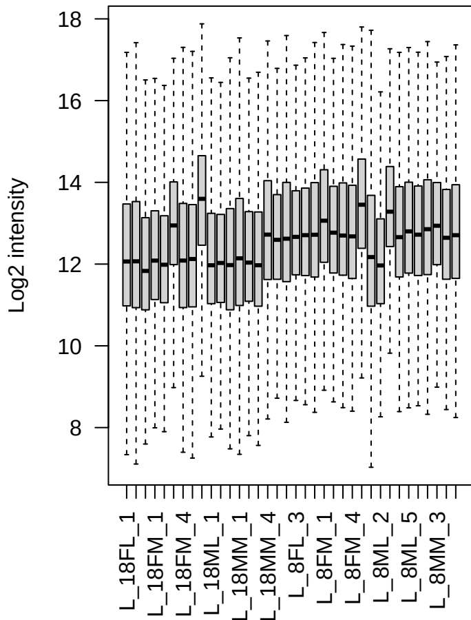
After VSN normalization
