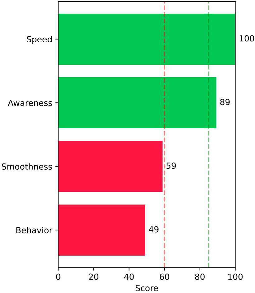
Component Scores
