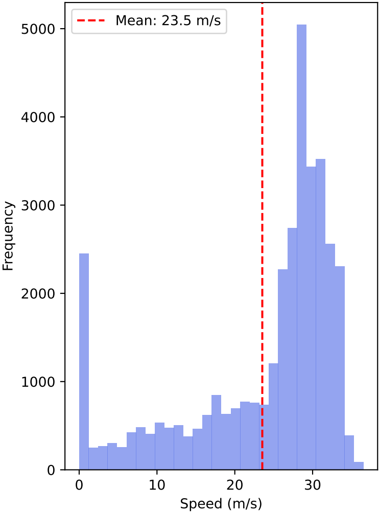
Speed Distribution
