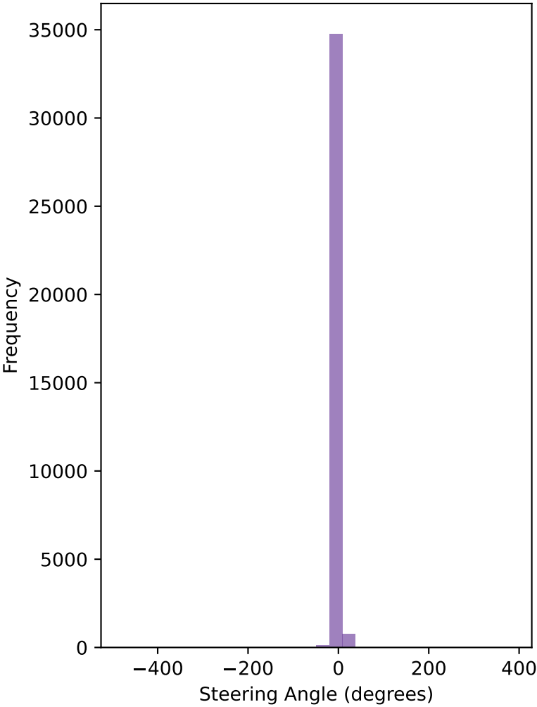
Steering Distribution
