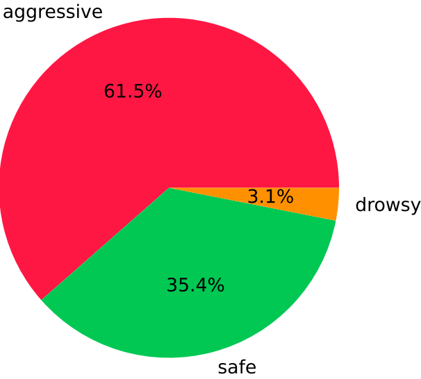
Behavior Distribution
