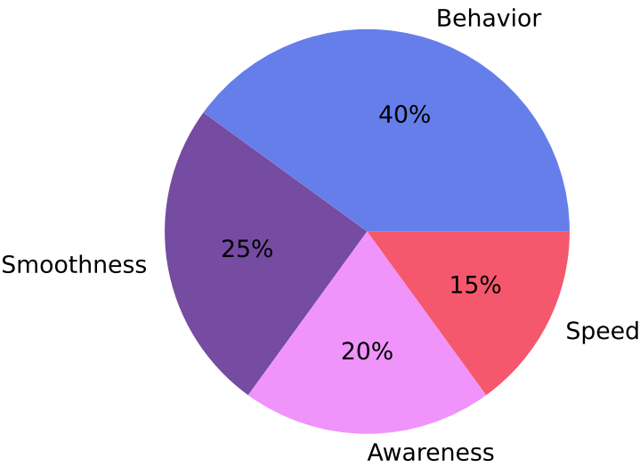
Score Weights
