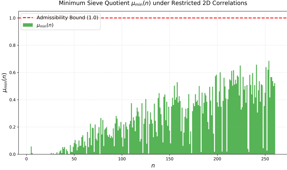
Figure 1: The minimum sieve quotient \mu_{\min}(n) under restricted 2D correlations. The upward trend indicates that pairwise interference struggles to maintain the admissibility bound \mu < 1 for larger n .
