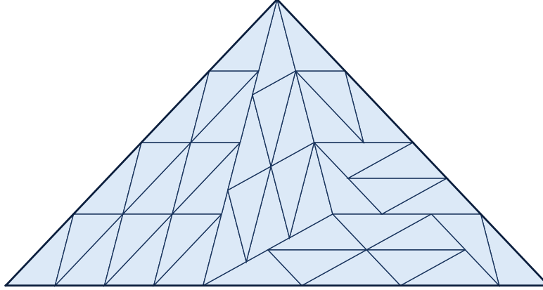
FIGURE 1. The 44-tiling of (16, 16, 22) by the tile (2, 3, 4) , found by exhaustive search and verified exactly. To our knowledge the first tiling in any of the three isosceles 3\alpha + 2\beta = \pi cases, and the smallest known triangle tiling in any incommensurable branch (the previously smallest was Herdt's 1215).
