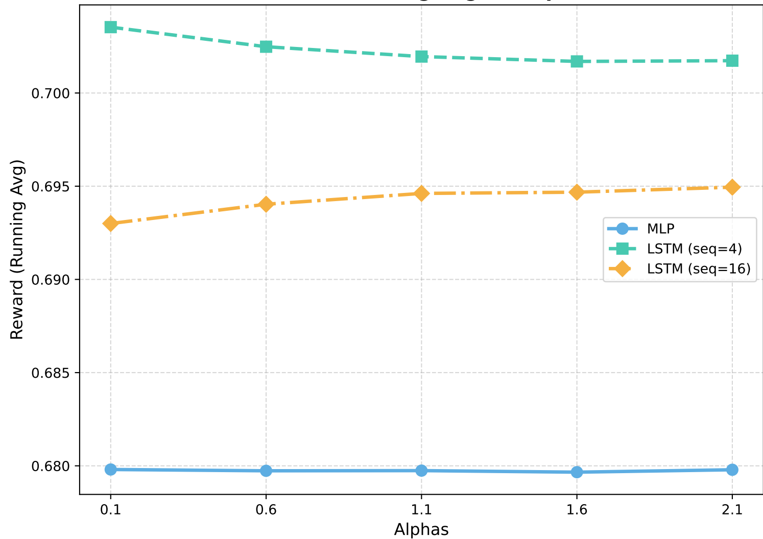
Reward (Running Avg) vs Alphas
