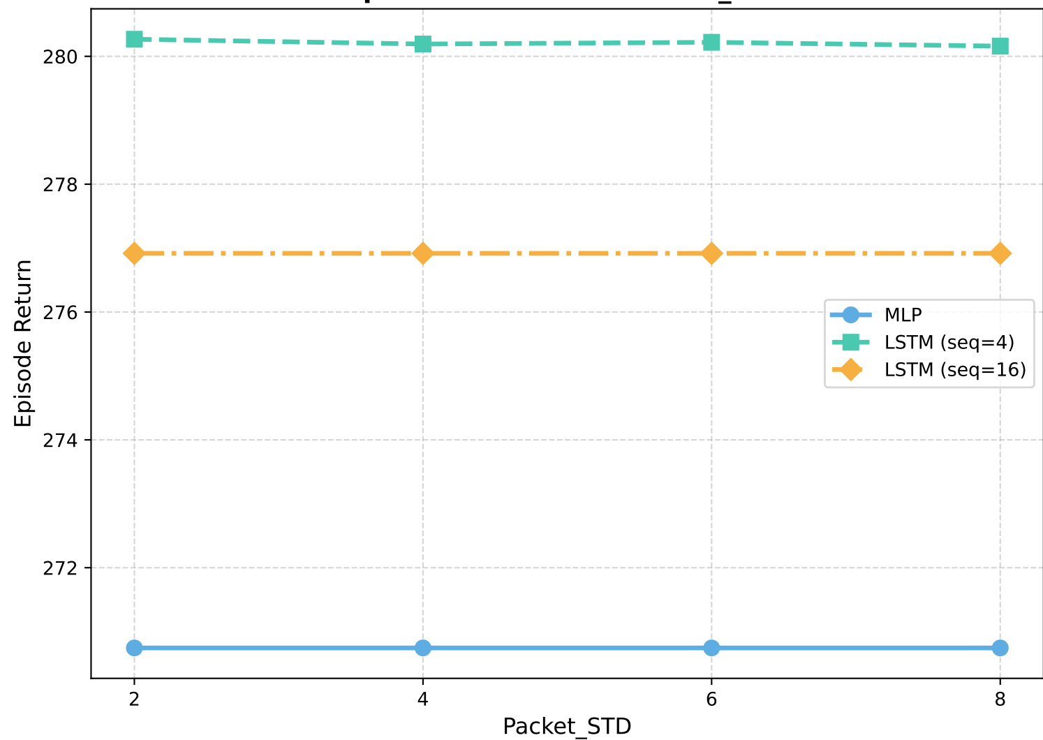
Episode Return vs Packet_STD
