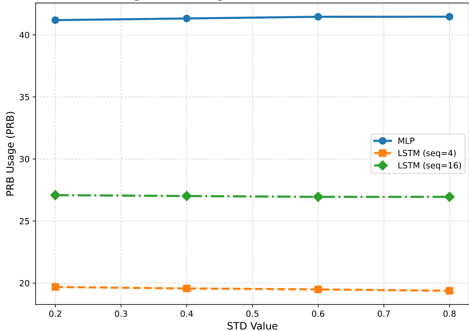
PRB Usage (PRB) (Avg: eMBB & URLLC) vs STD Value
