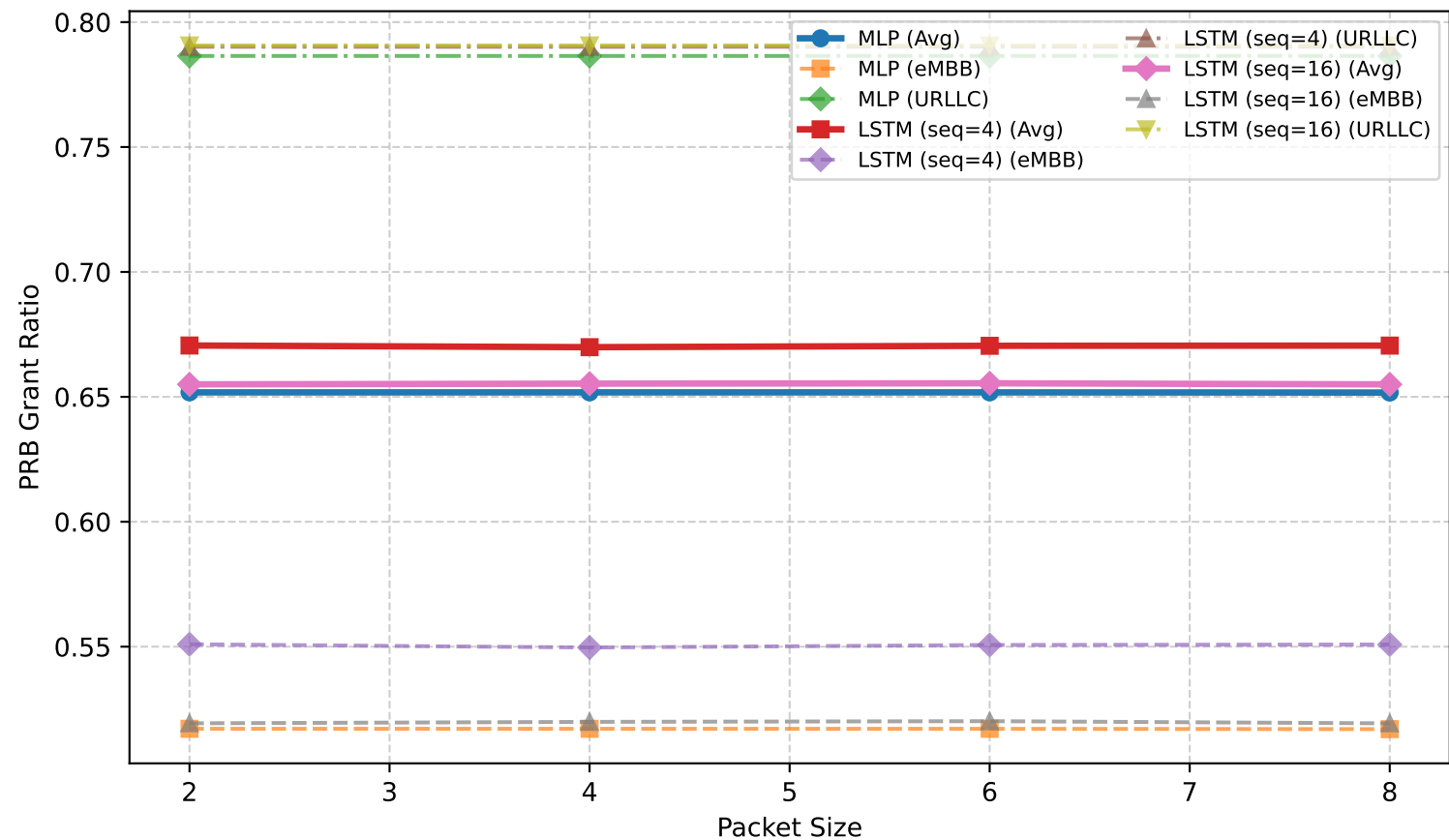
PRB Grant Ratio vs Packet Size
