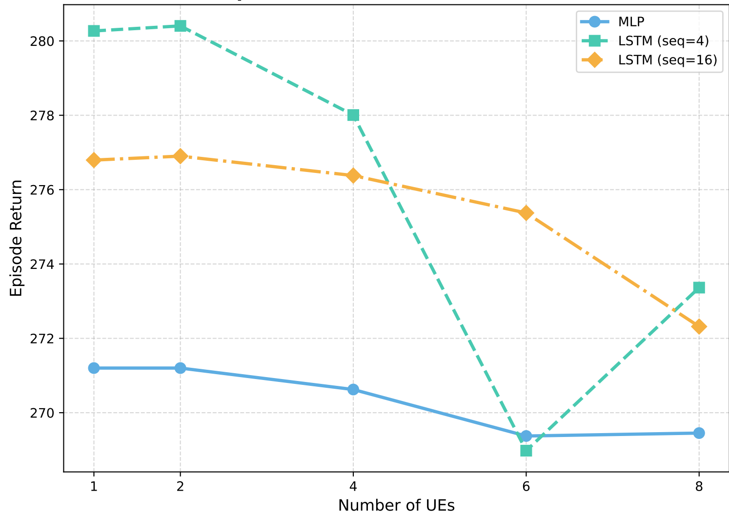
Episode Return vs Number of UEs
