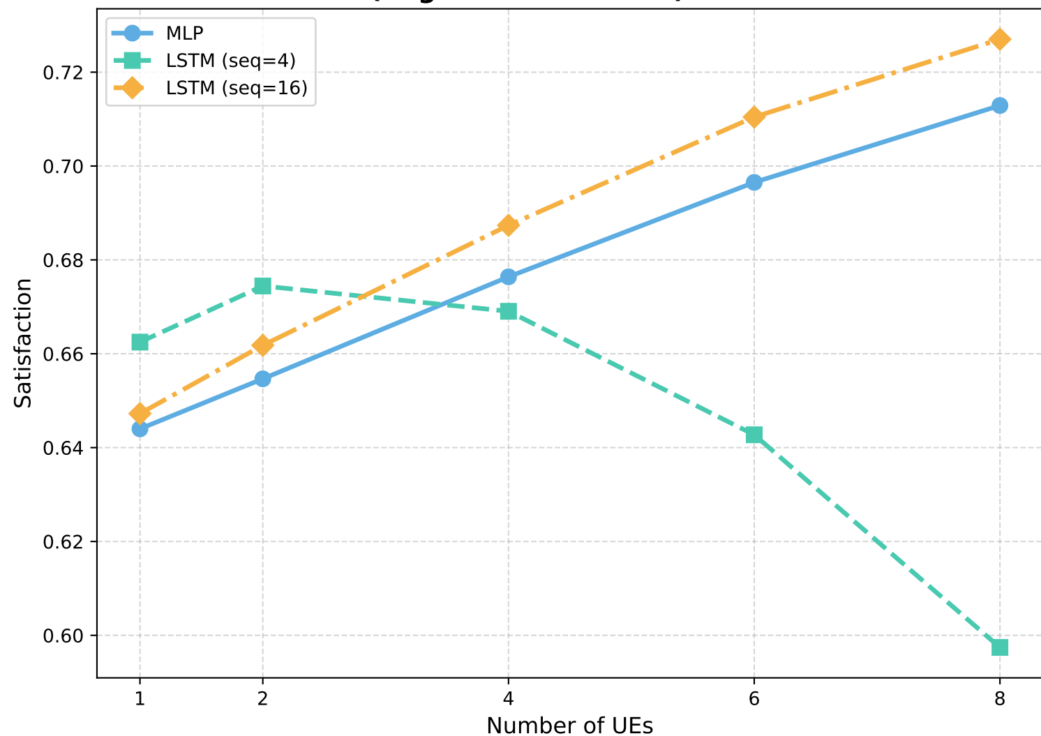
Satisfaction (Avg: eMBB & URLLC) vs Number of UEs
