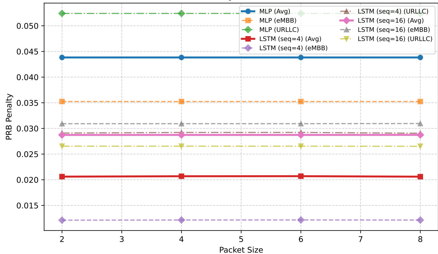
PRB Penalty vs Packet Size
