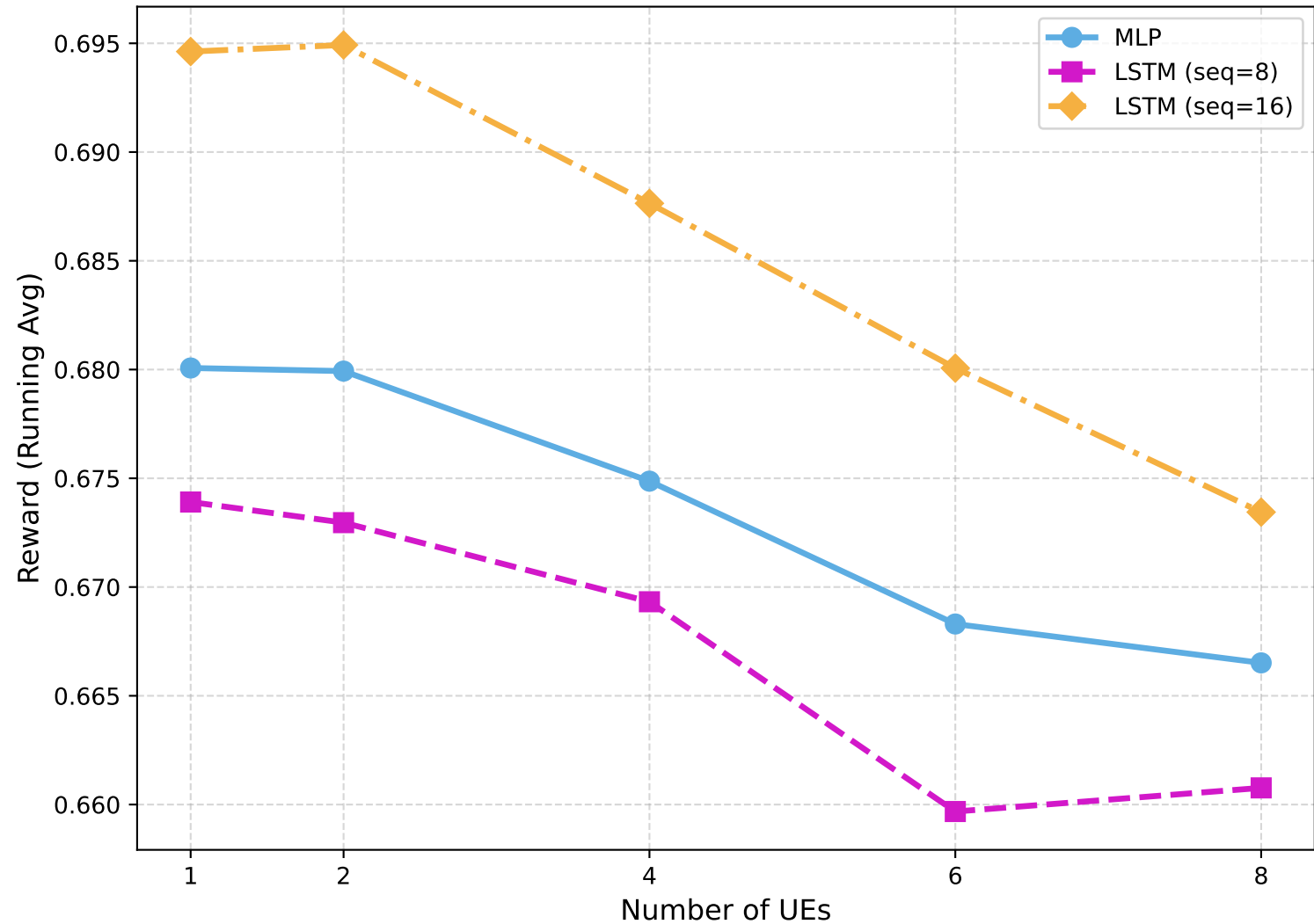
Reward (Running Avg) vs Number of UEs
