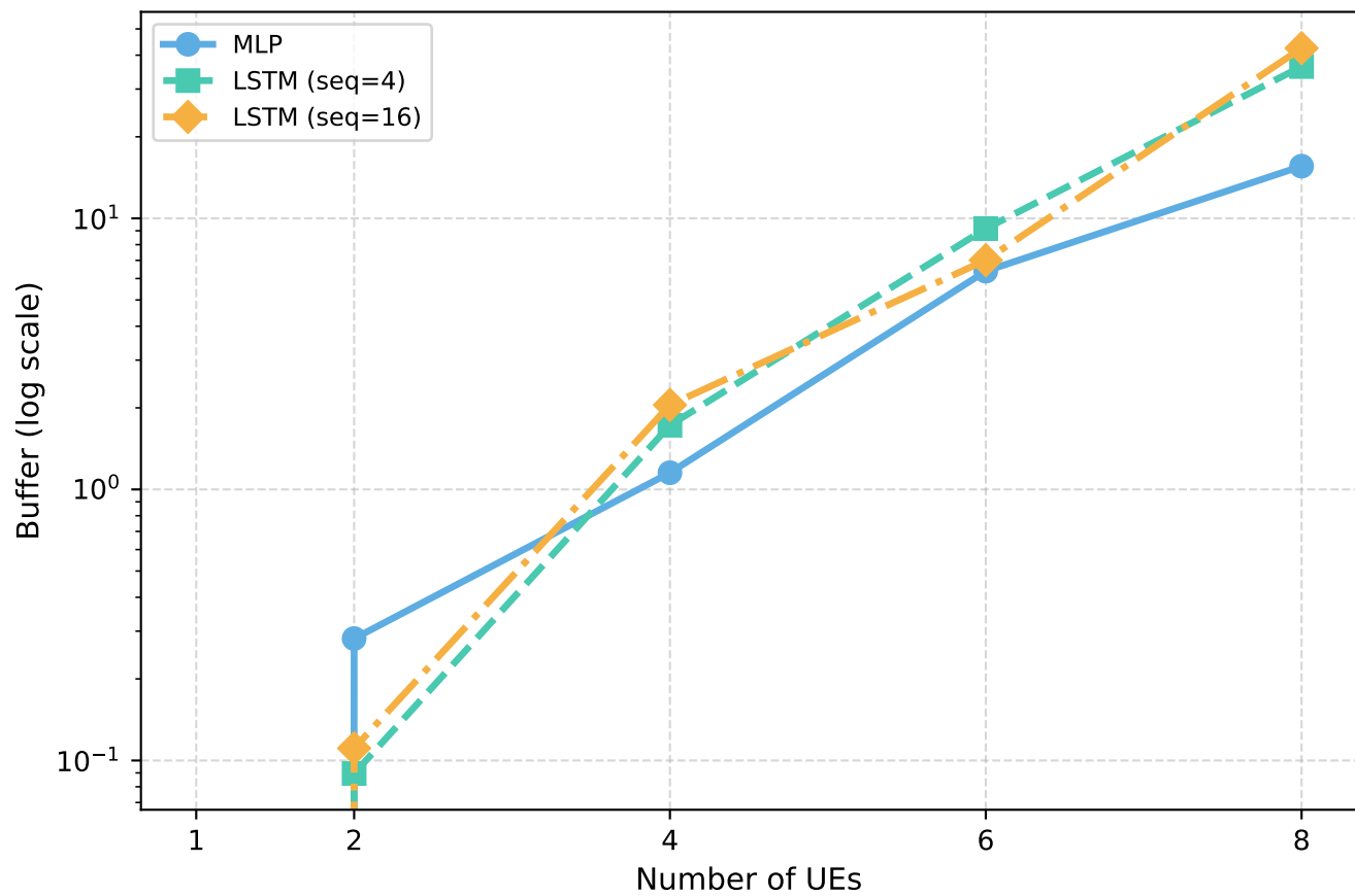
Buffer - URLLC
