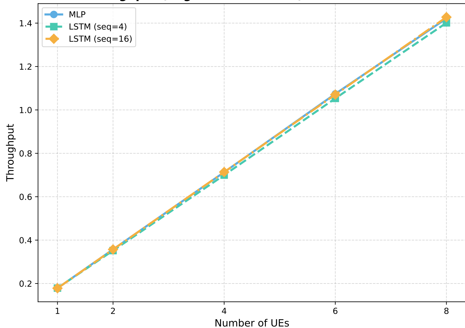
Throughput (Avg: eMBB & URLLC) vs Number of UEs
