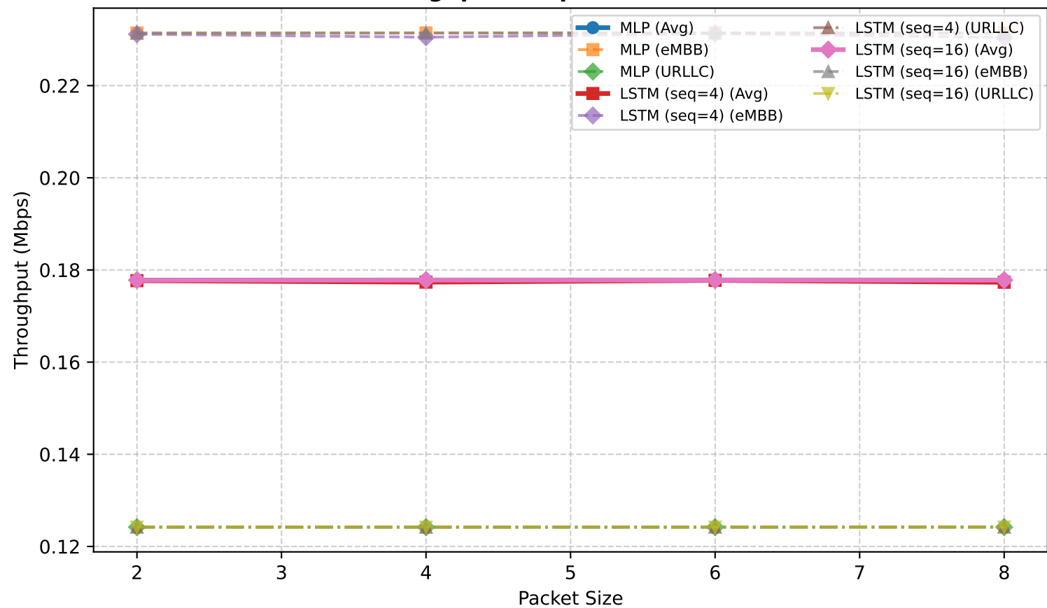
Throughput (Mbps) vs Packet Size
