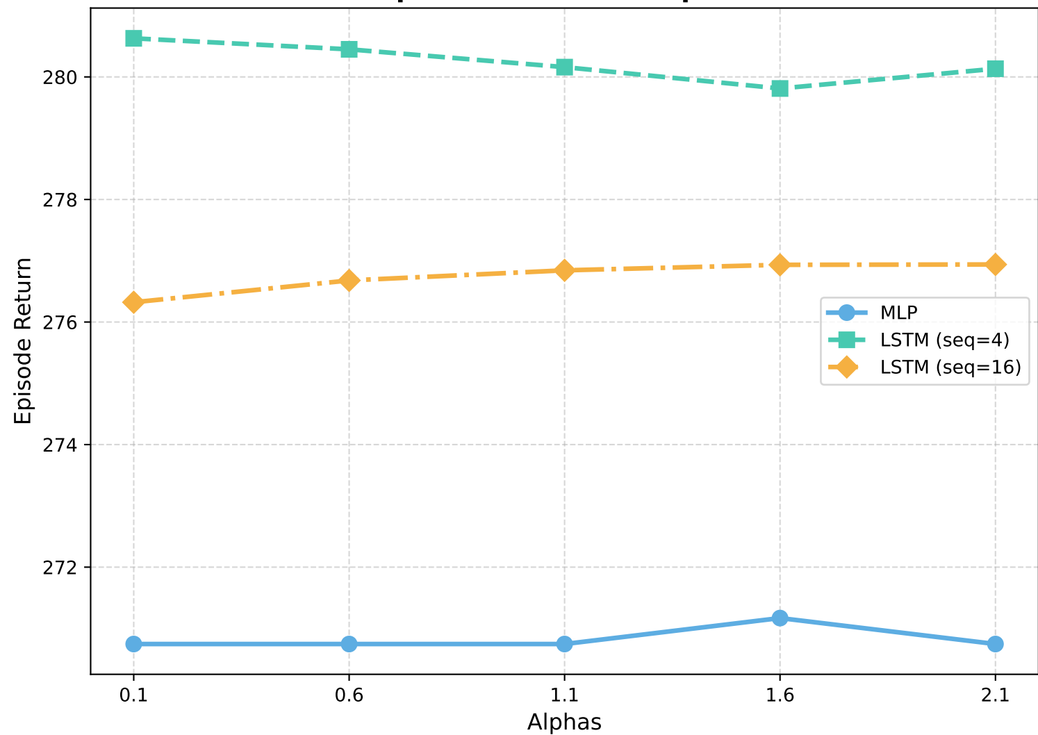
Episode Return vs Alphas
