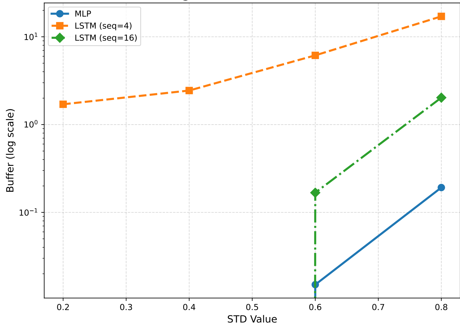
Buffer (Avg: eMBB & URLLC) vs STD Value
