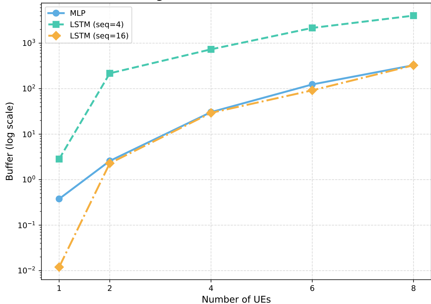
Buffer (Avg: eMBB & URLLC) vs Number of UEs
