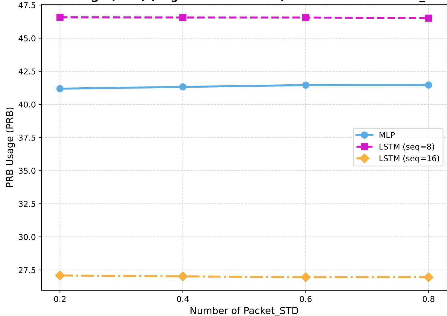
PRB Usage (PRB) (Avg: eMBB & URLLC) vs Number of Packet_STD
