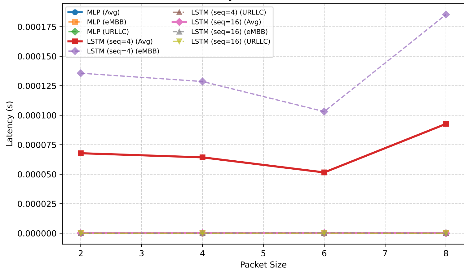
Latency (s) vs Packet Size
