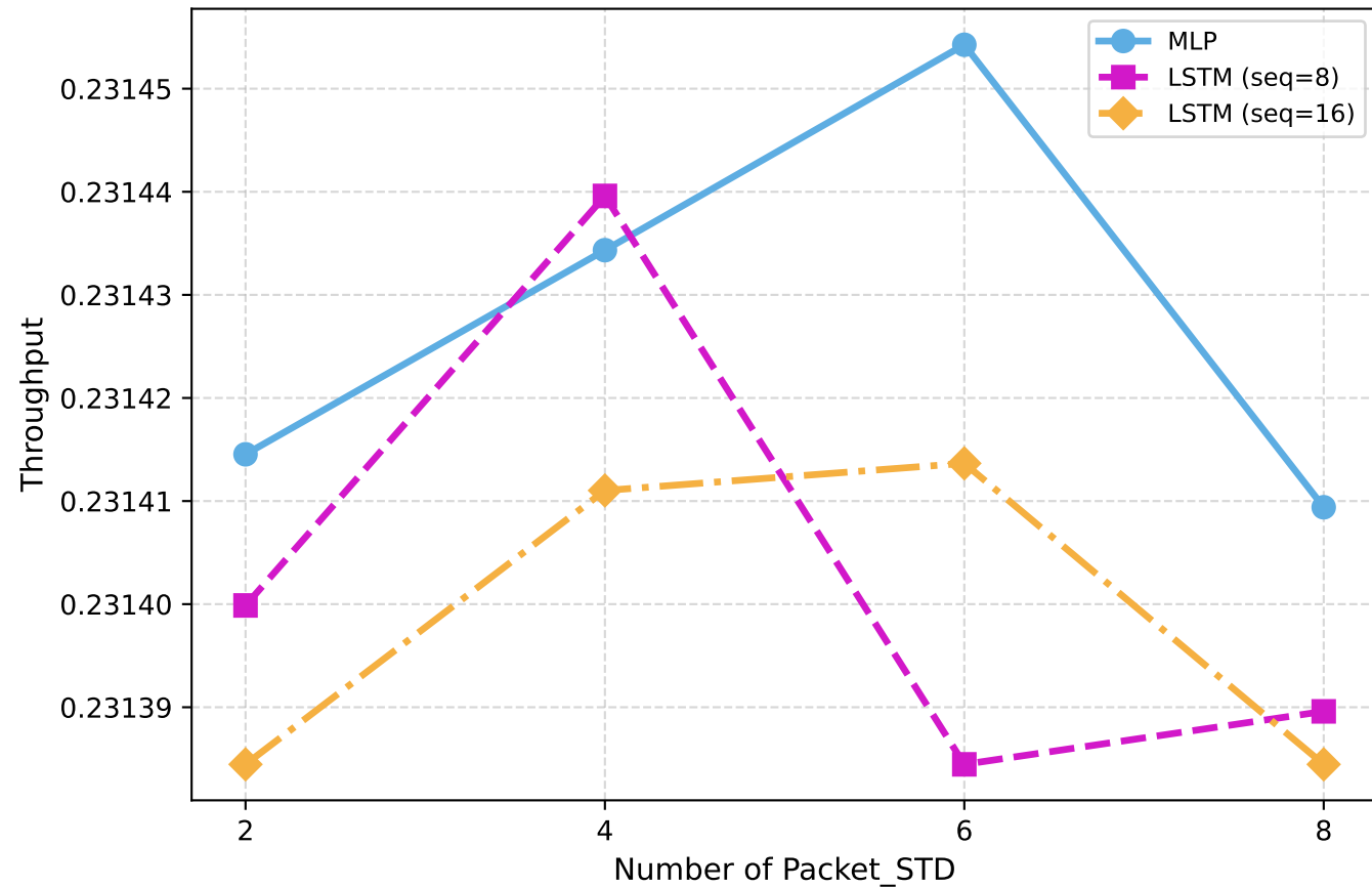
Throughput - eMBB
