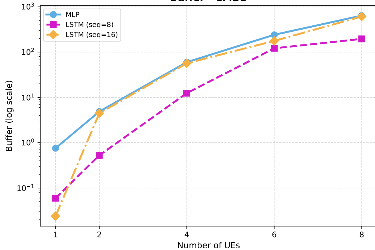
Buffer - eMBB
