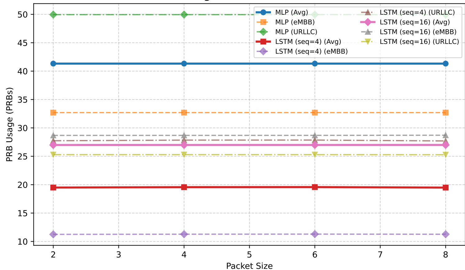
PRB Usage (PRBs) vs Packet Size
