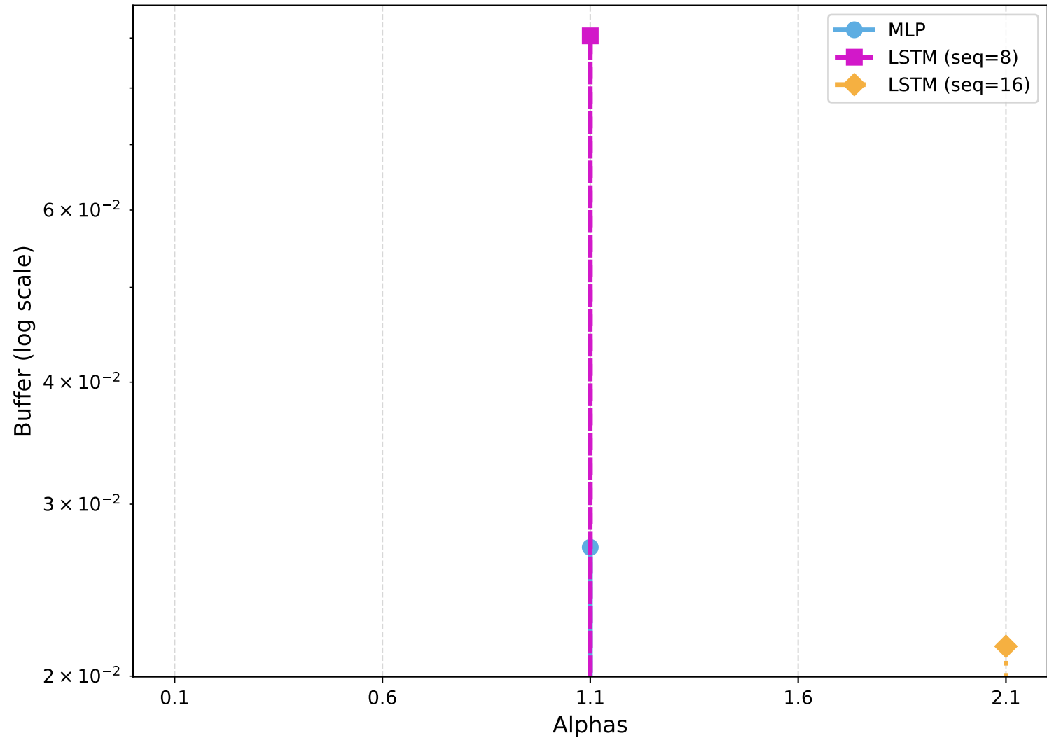
Buffer (Avg: eMBB & URLLC) vs Alphas
