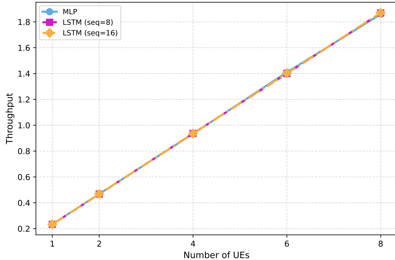
Throughput - eMBB
