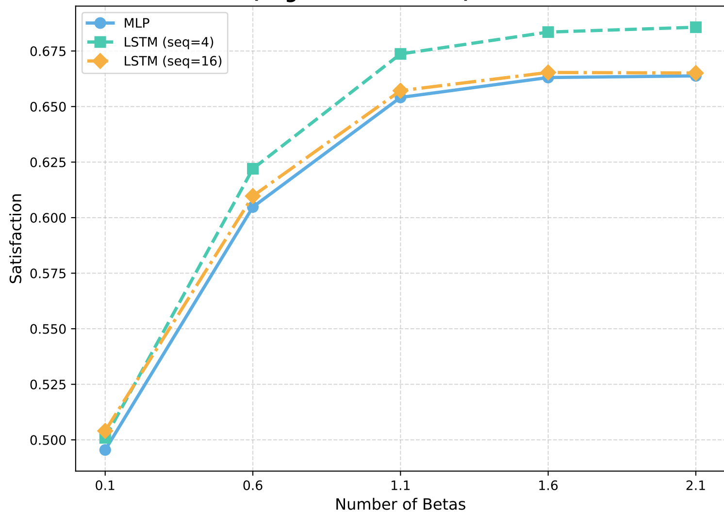
Satisfaction (Avg: eMBB & URLLC) vs Number of Betas
