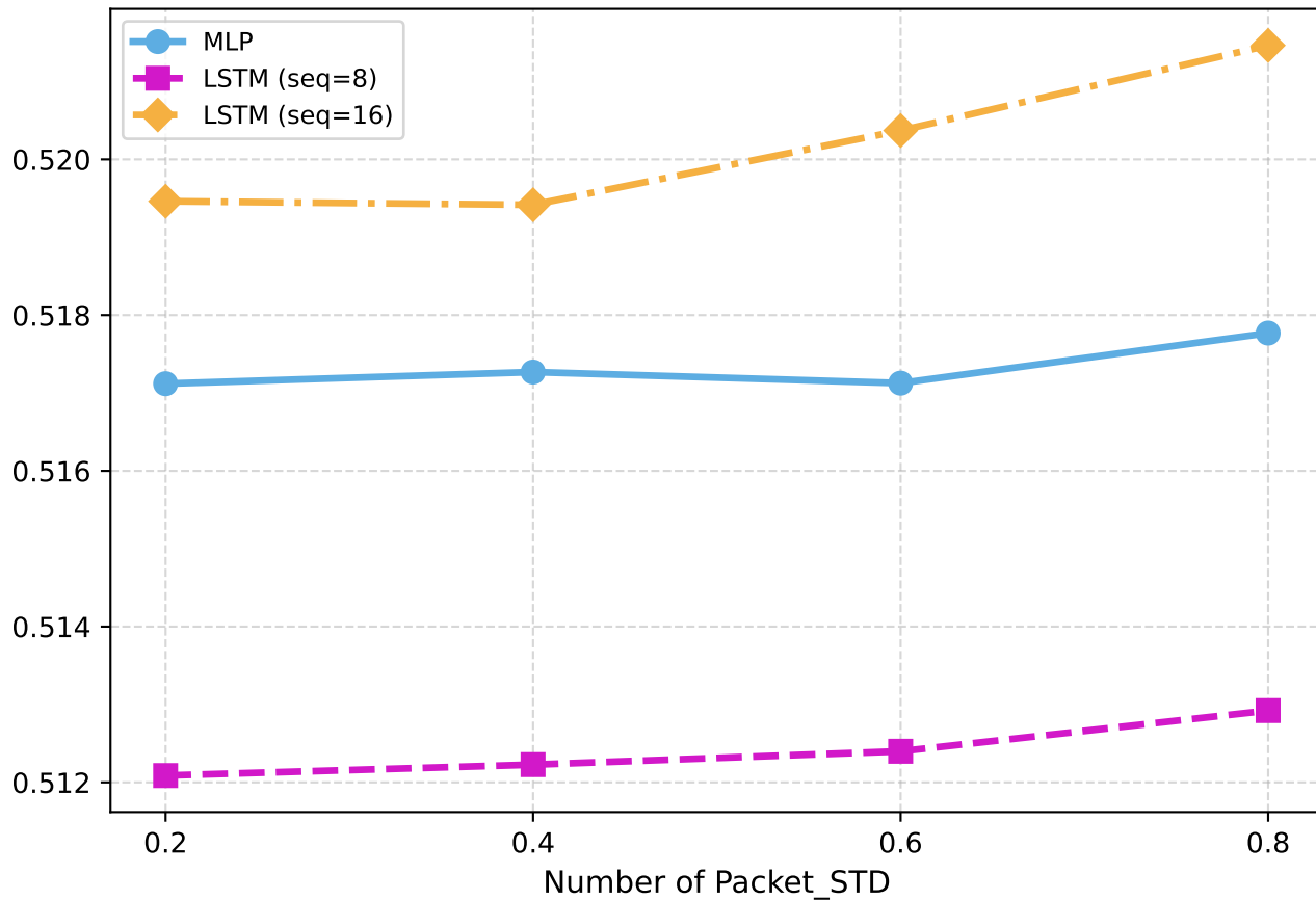
Satisfaction - eMBB
