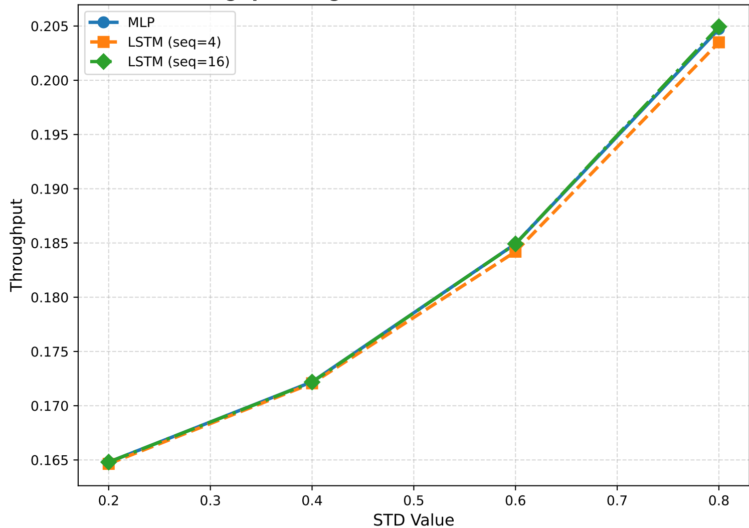
Throughput (Avg: eMBB & URLLC) vs STD Value
