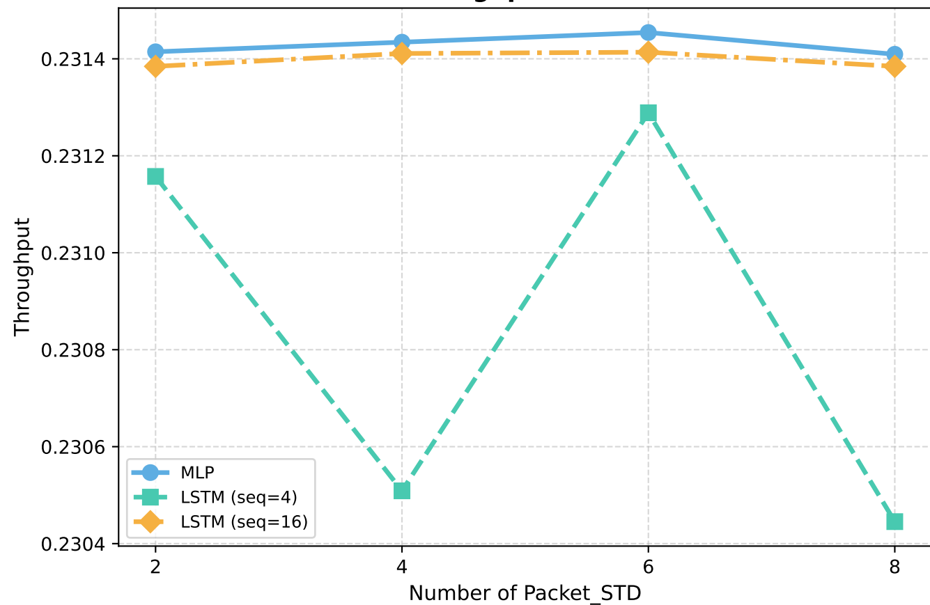
Throughput - eMBB
