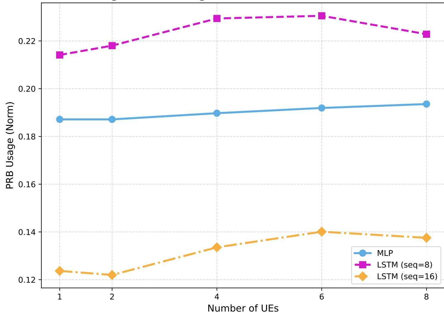
PRB Usage (Norm) (Avg: eMBB & URLLC) vs Number of UEs
