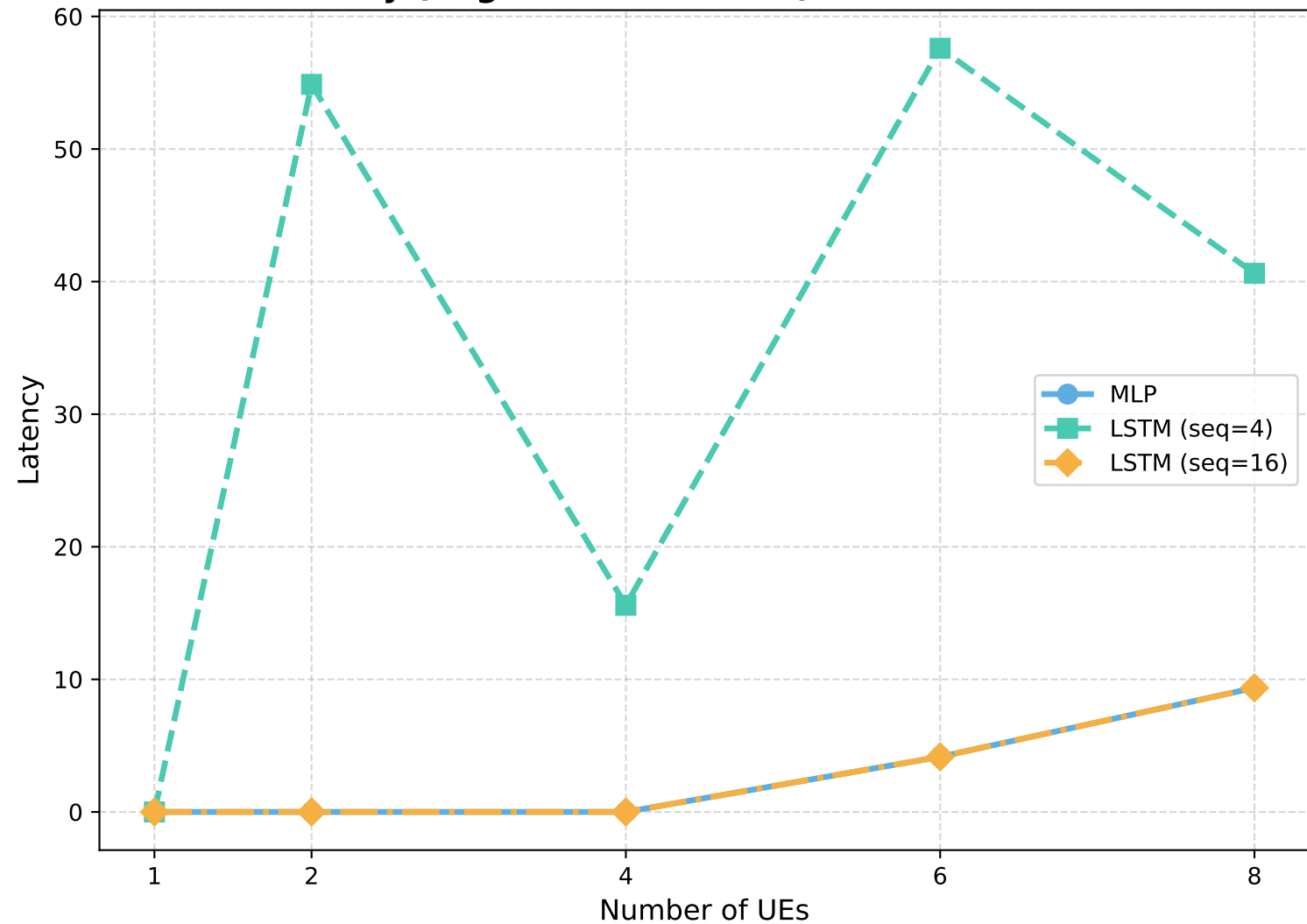
Latency (Avg: eMBB & URLLC) vs Number of UEs
