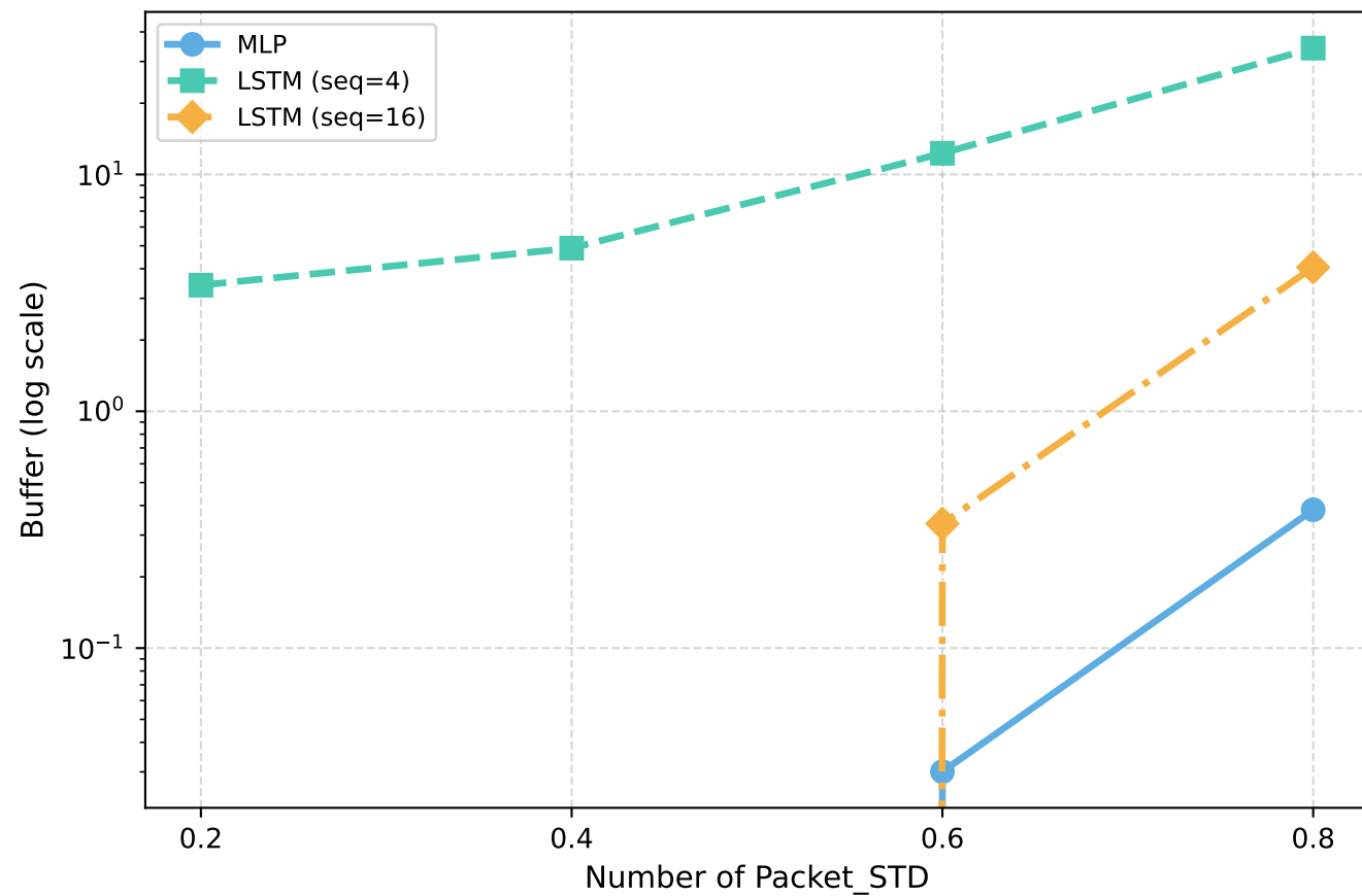
Buffer - eMBB
