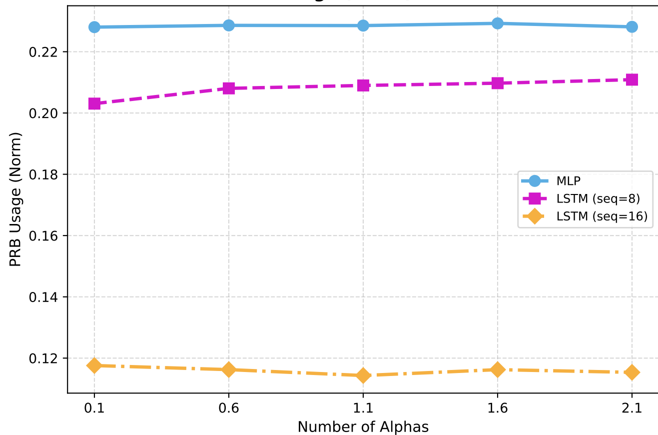
PRB Usage (Norm) - URLLC
