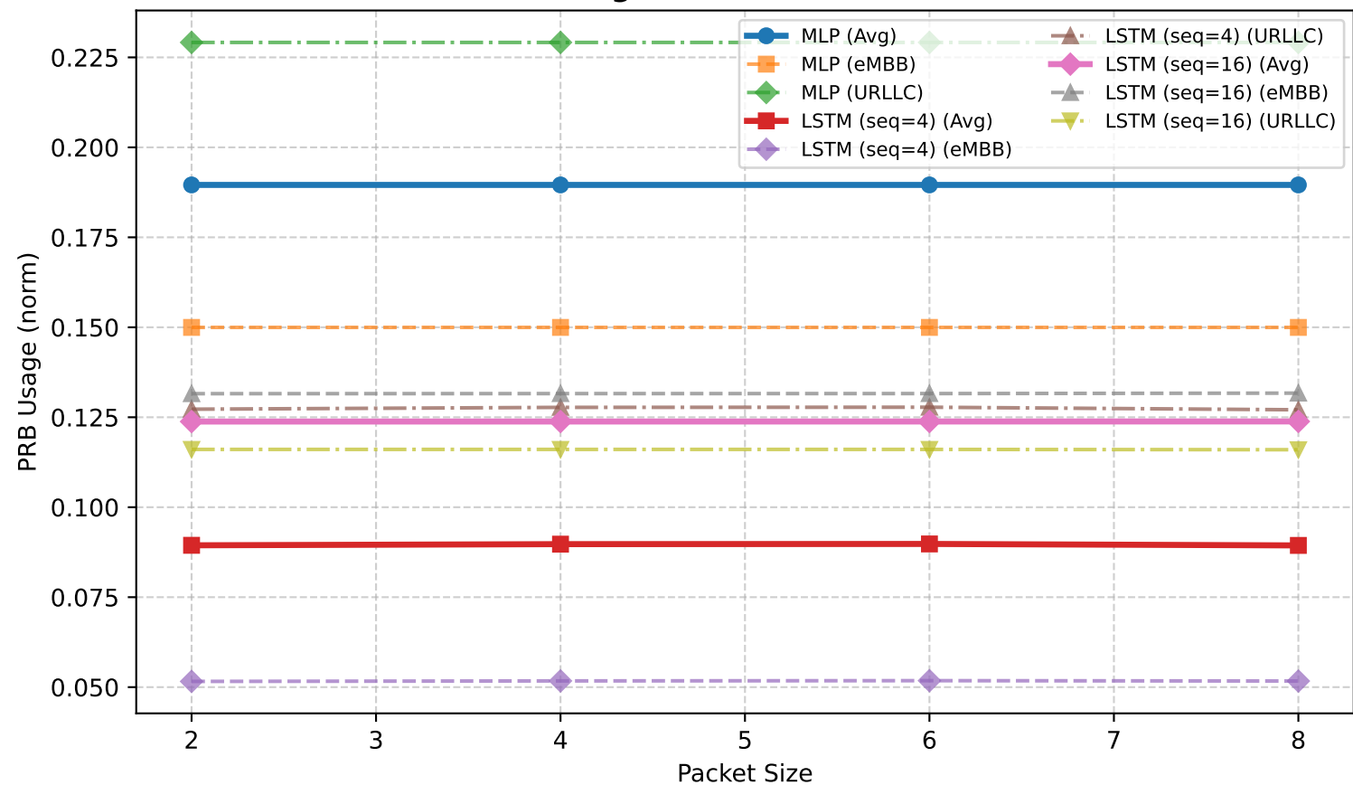
PRB Usage (norm) vs Packet Size
