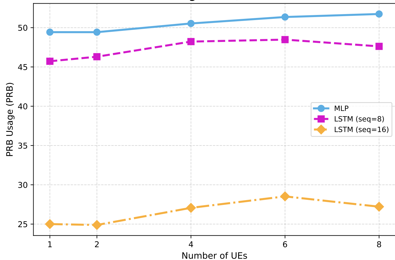
PRB Usage (PRB) - URLLC
