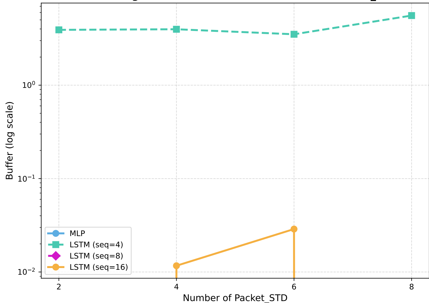
Buffer (Avg: eMBB & URLLC) vs Number of Packet_STD
