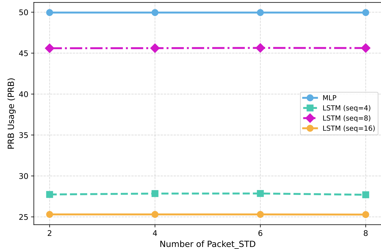
PRB Usage (PRB) - URLLC
