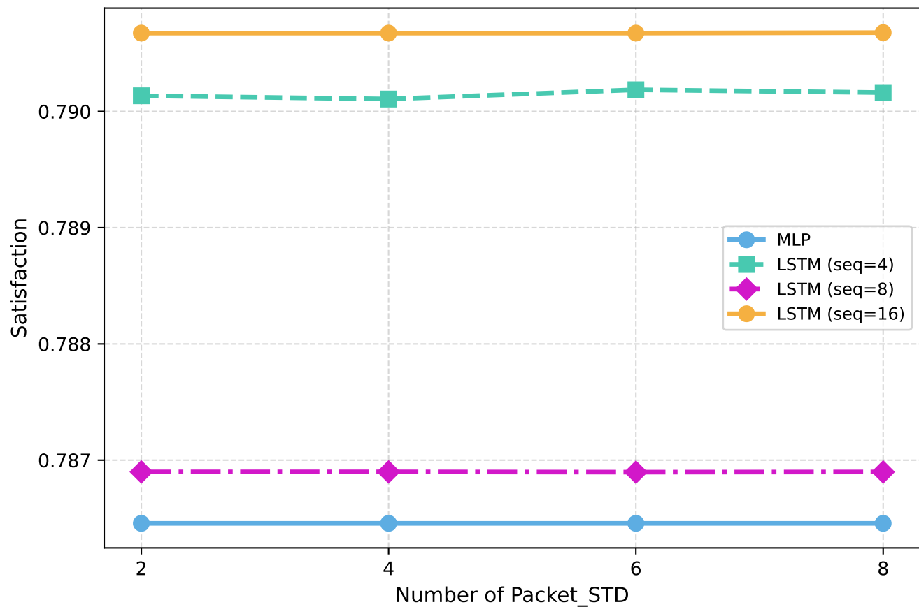
Satisfaction - URLLC
