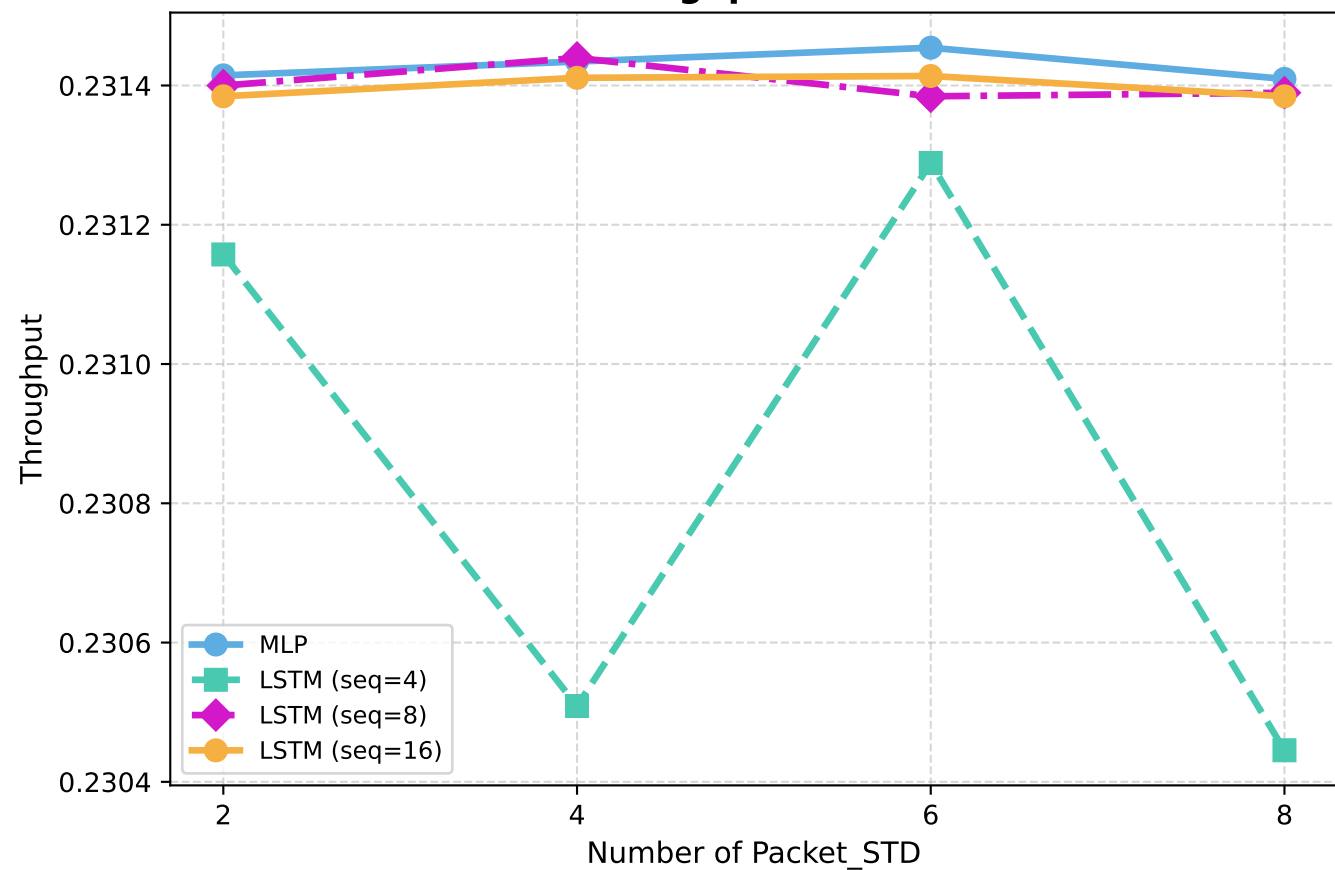
Throughput - eMBB
