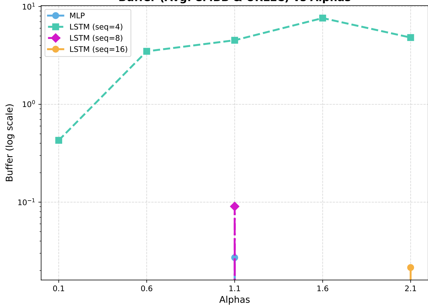
Buffer (Avg: eMBB & URLLC) vs Alphas
