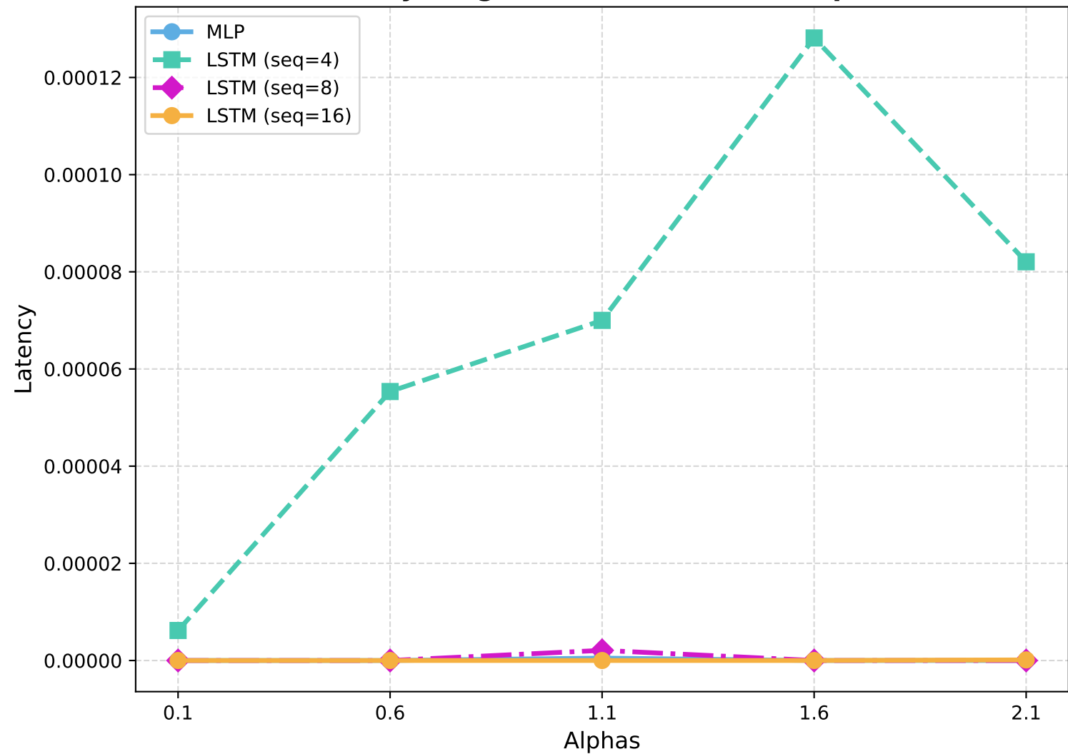
Latency (Avg: eMBB & URLLC) vs Alphas
