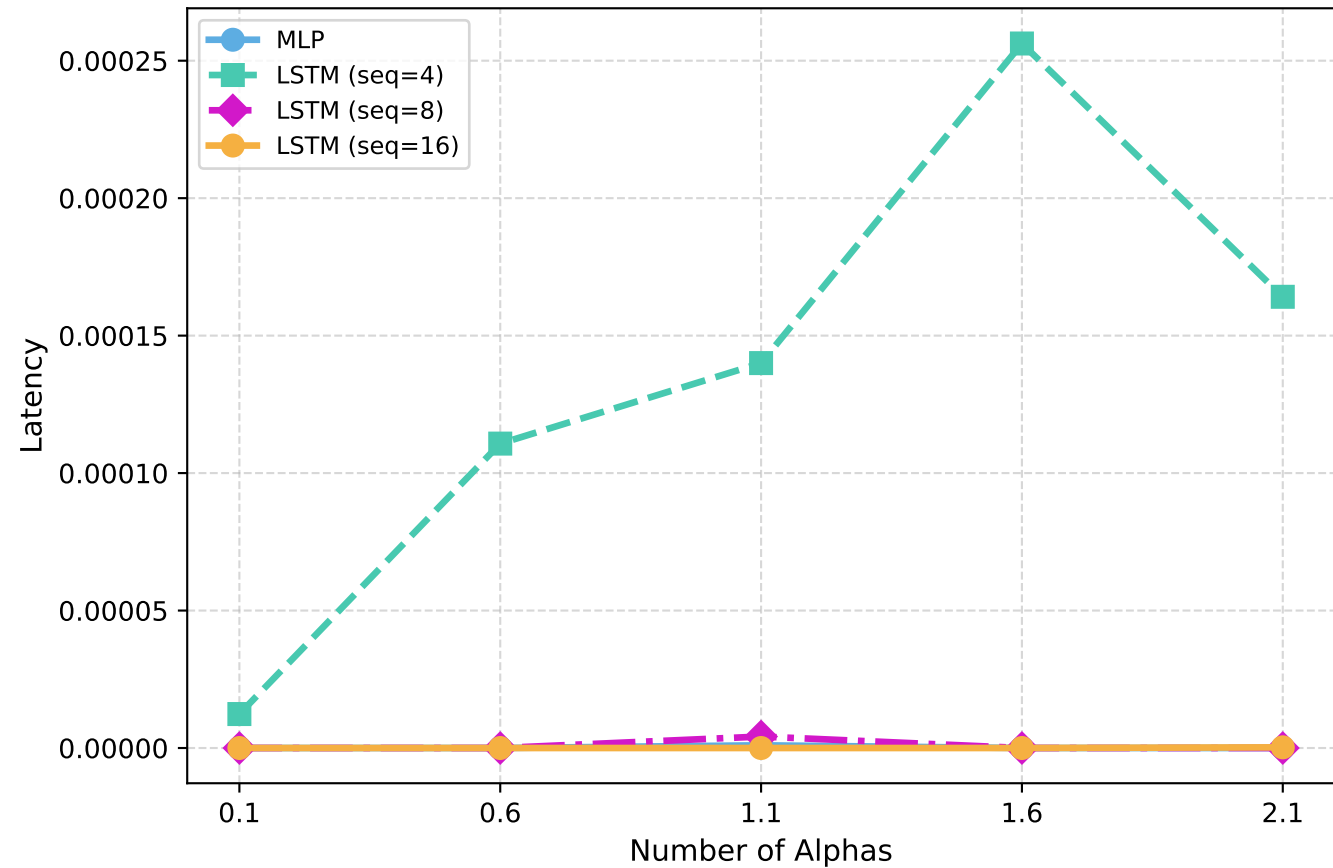
Latency - eMBB
