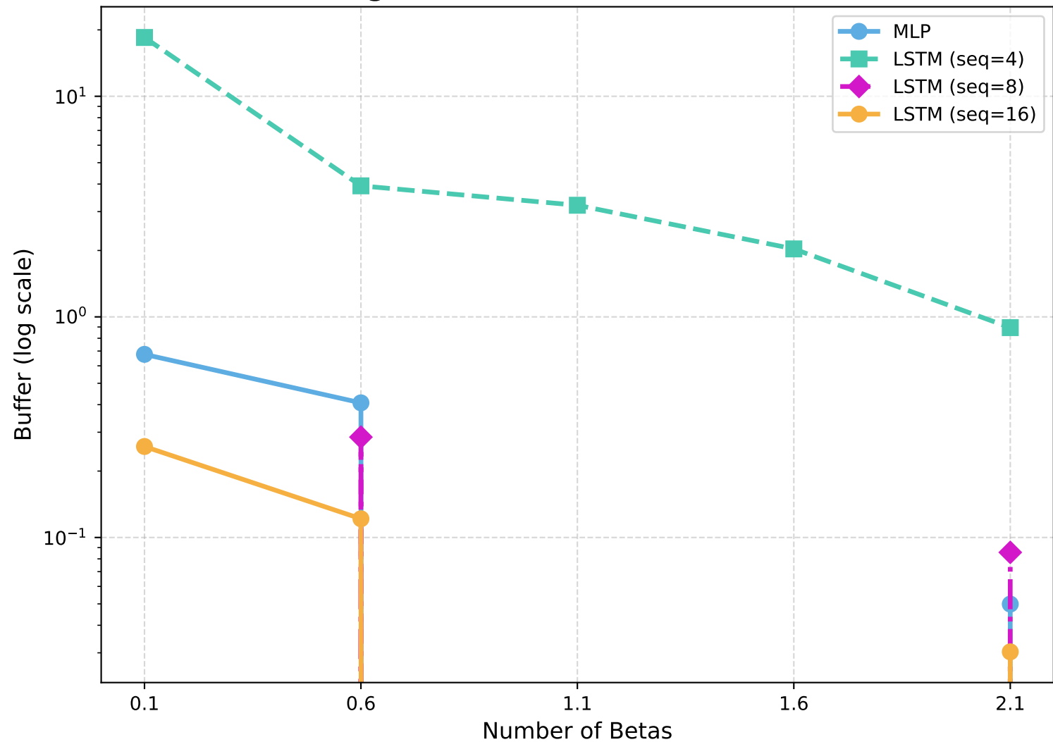
Buffer (Avg: eMBB & URLLC) vs Number of Betas
