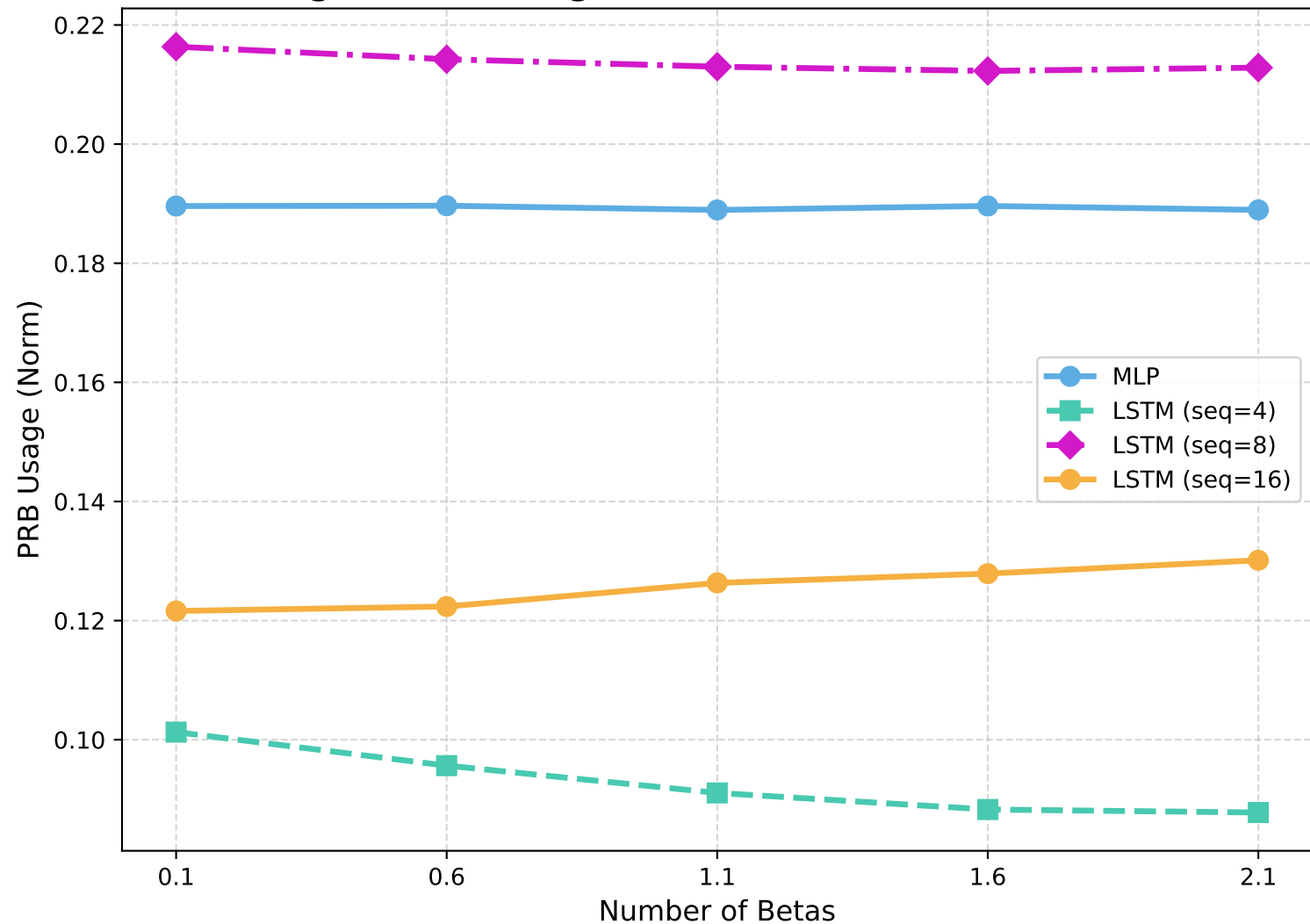
PRB Usage (Norm) (Avg: eMBB & URLLC) vs Number of Betas
