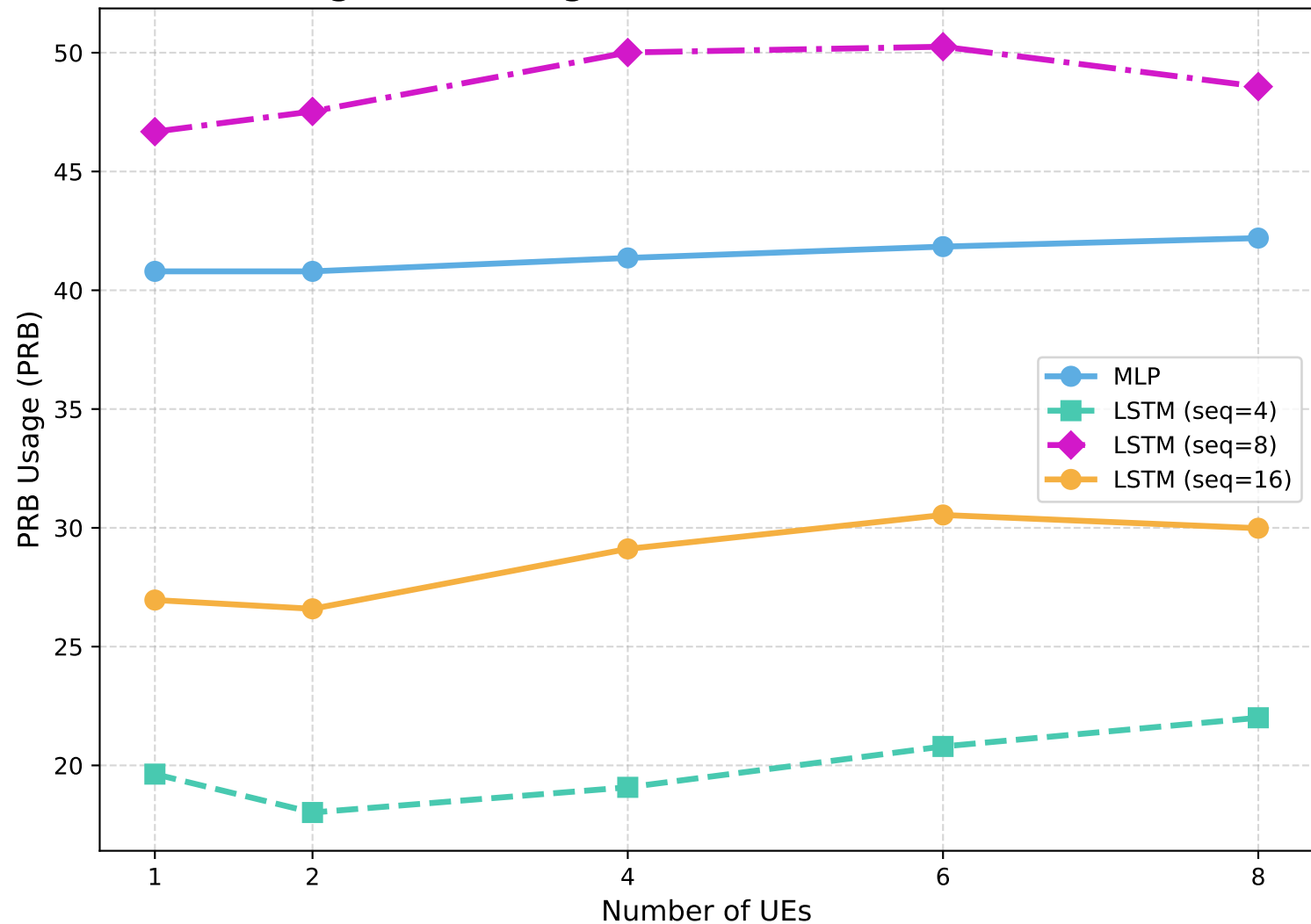
PRB Usage (PRB) (Avg: eMBB & URLLC) vs Number of UEs
