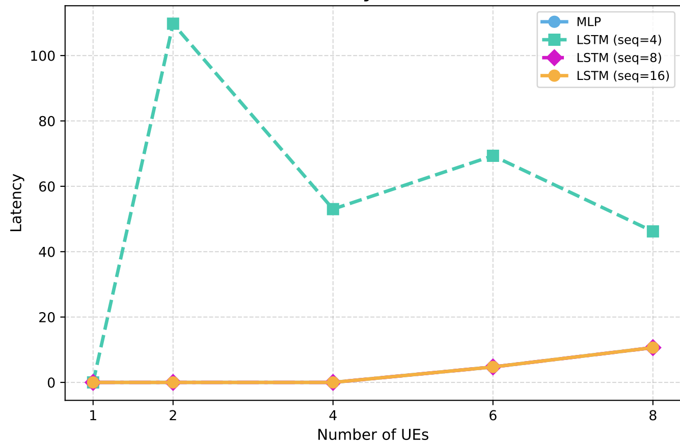
Latency - eMBB
