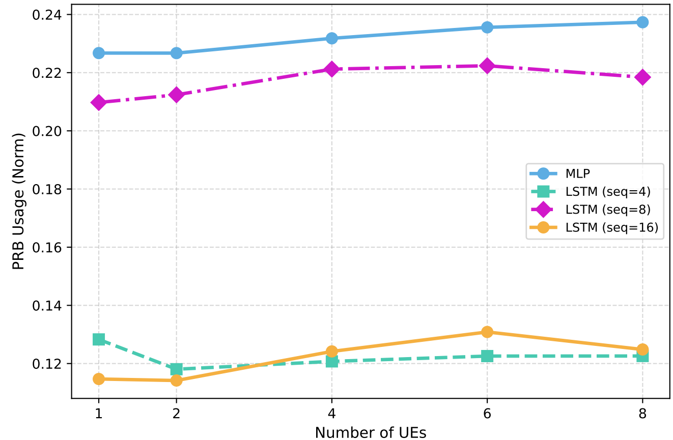
PRB Usage (Norm) - URLLC
