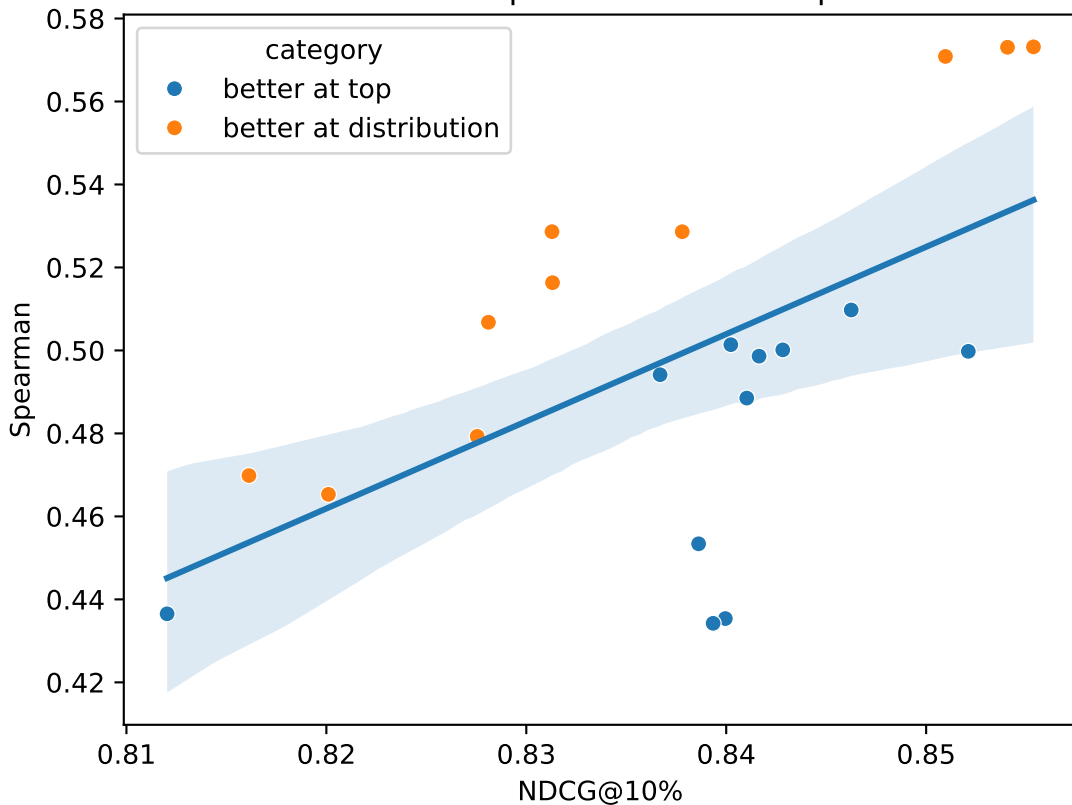
median NDCG top 10% vs median Spearman
