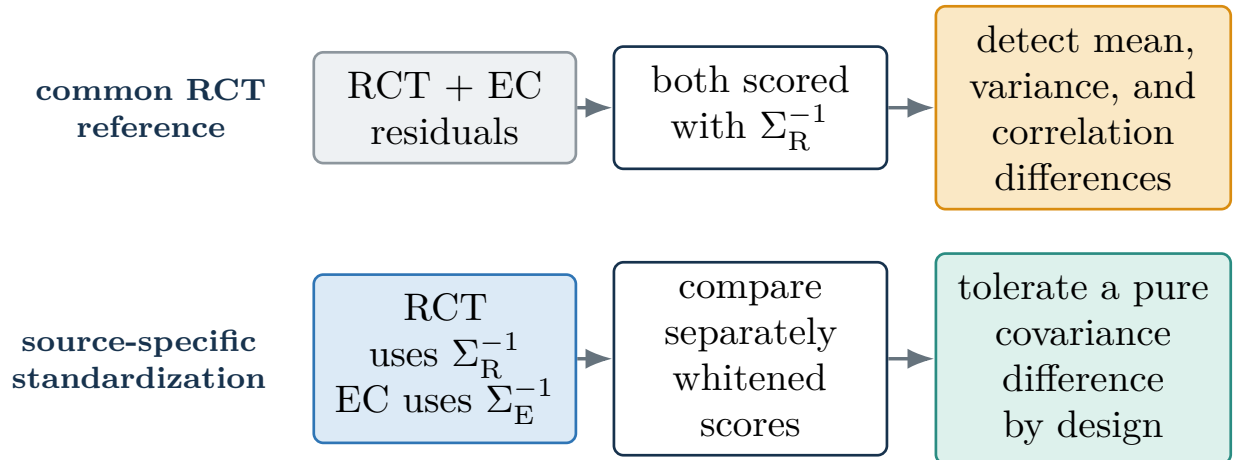
Figure 6: Common-reference and source-specific standardization answer different questions. The latter can intentionally normalize away a pure covariance difference, but its estimated external covariance can also absorb contamination.
