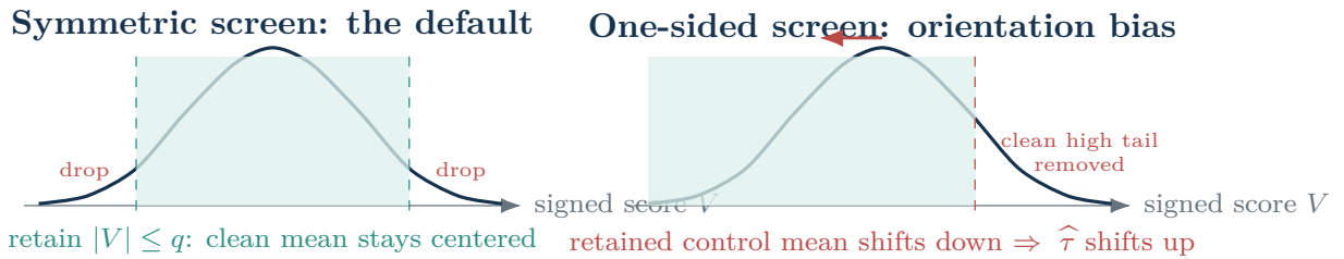
Figure 9: Why the carried-forward default is symmetric. When the score is aligned with the estimand, asymmetric deletion of clean scores changes the retained clean outcome mean and therefore biases the treatment-effect estimate.
