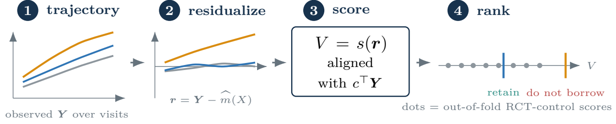
Figure 4: From an observed longitudinal record to a borrowing decision. The working model removes the expected covariate-specific course and defines a useful ordering; out-of-fold randomized controls empirically calibrate how extreme that ordering is.
