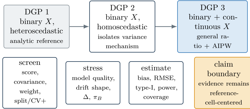
Figure 11: The simulation program moves from an analytically transparent mechanism study to a more general covariate and estimator structure. It is designed to isolate one failure mode at a time rather than to mimic a clinical dataset immediately.
