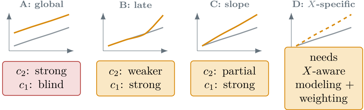
Figure 5: Score choice is a scientific design choice. A contrast score is intentionally sensitive to drift that projects onto its estimand and can be blind to orthogonal drift; an omnibus score sees more trajectory differences but can exclude controls that are harmless for the target mean contrast.
