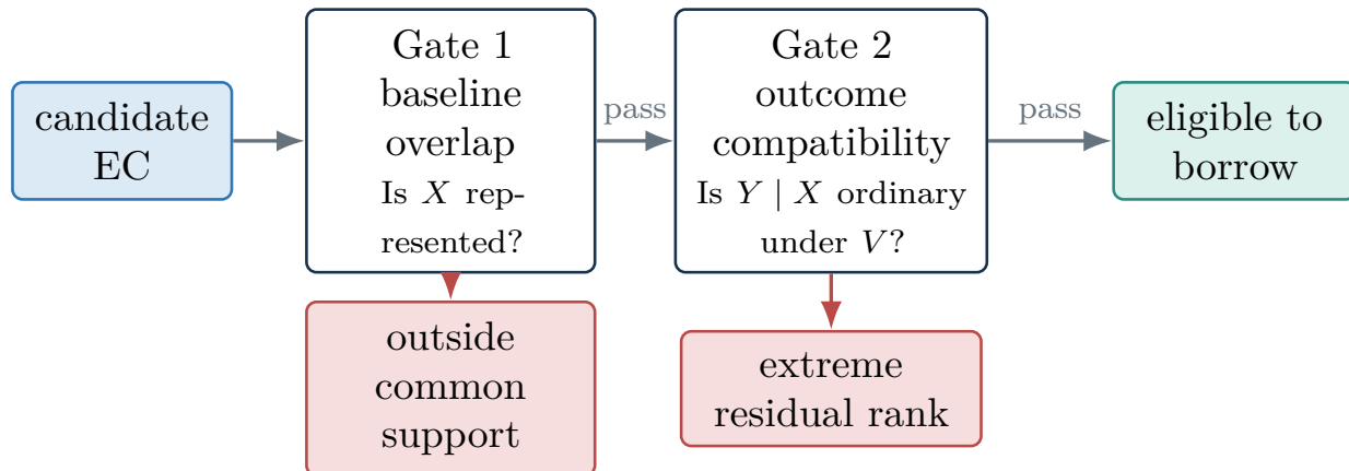
Figure 2: Baseline support and outcome compatibility are separate gates. Propensity-based tools address the first; the proposed residual-rank diagnostic addresses the second.
