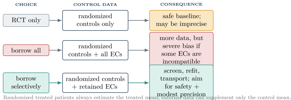
Figure 1: The statistical decision in one picture. The randomized treated arm always estimates the treated mean; the methodological question is how much external information may safely supplement the randomized control mean.
