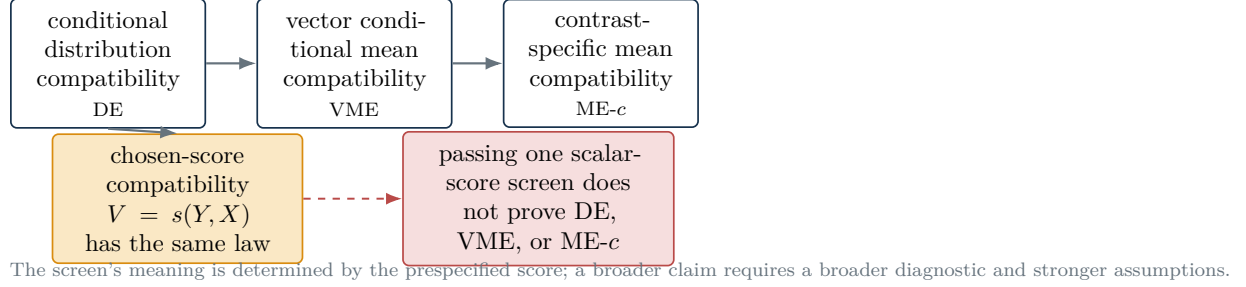
Figure 3: Compatibility targets and the claim boundary. A scalar score is a deliberately lossy diagnostic summary; passing its screen is not evidence for every stronger notion above it.
