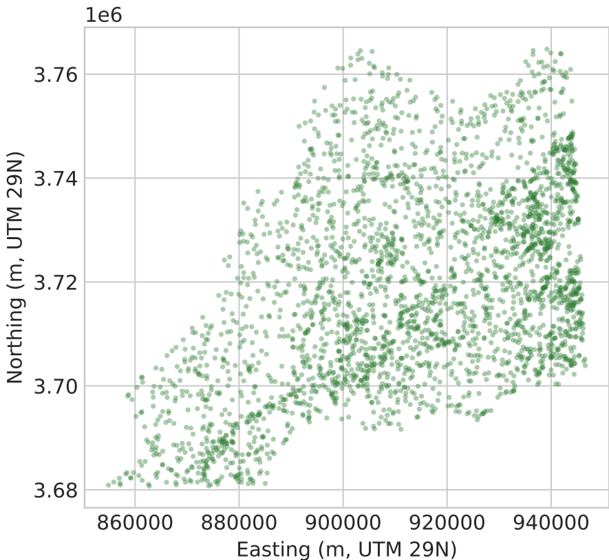
Figure 2. Study area -- Allal El Fassi sub-watershed sample distribution (Sebou Basin, Morocco; EPSG:32629)
