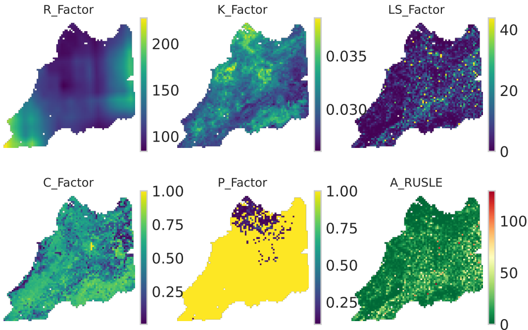
Figure 3. RUSLE factor maps
