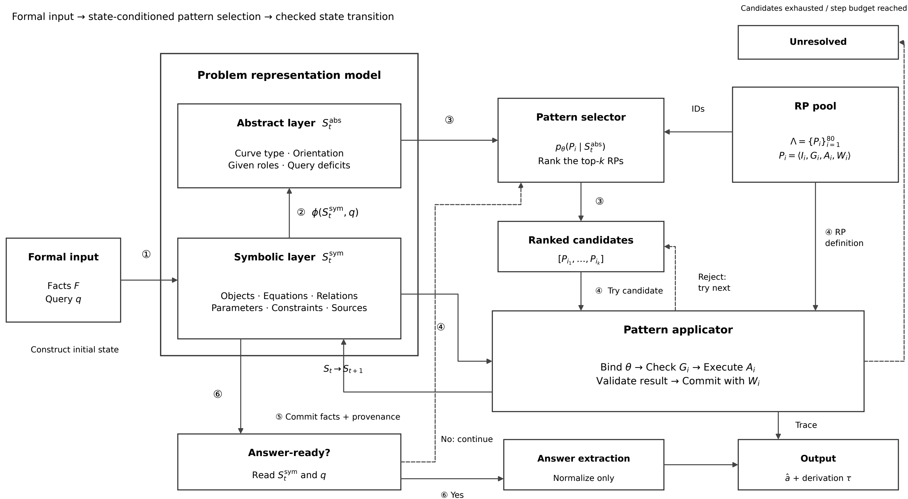
Fig. 2 | Conic-Solver: framework sketch
