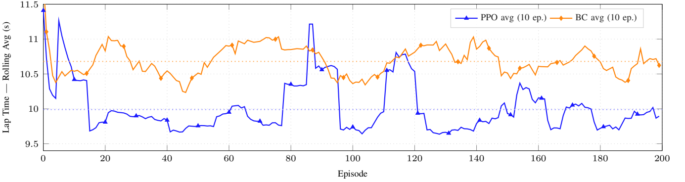
Fig. 2. Lap time per inference episode for PPO ( n = 198 ) and BC ( n = 172 ). Markers placed every 10 episodes. Failed episodes are excluded (PPO: 3, BC: 28). PPO outliers up to 18.33 s reflect occasional policy instability.
