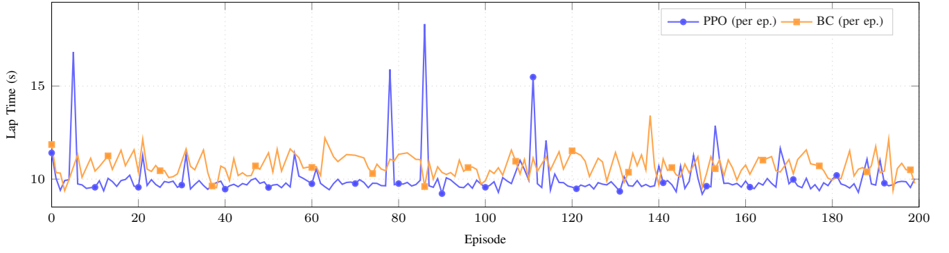
Fig. 2. Lap time per inference episode for PPO ( n = 198 ) and BC ( n = 172 ). Markers placed every 10 episodes. Failed episodes are excluded (PPO: 3, BC: 28). PPO outliers up to 18.33 s reflect occasional policy instability.
