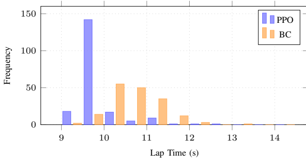
Fig. 4. Lap time frequency distribution for PPO and BC (successful episodes only, bin width = 0.5 s). PPO bin 9.5–10.0 s contains 142 episodes (71.7%). PPO outliers > 14.5 s (4 episodes) are excluded for clarity.
