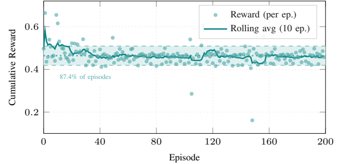
Fig. 5. PPO cumulative reward per inference episode with 10-episode rolling average. The shaded band marks mean \pm 1 std ( \mu = 0.464 , \sigma = 0.045 ), containing 87.4% of episodes, indicating a stable converged policy.
